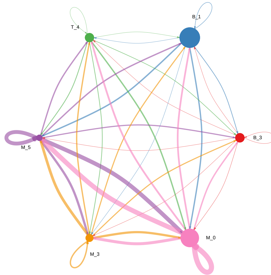
Interaction weights/strength
