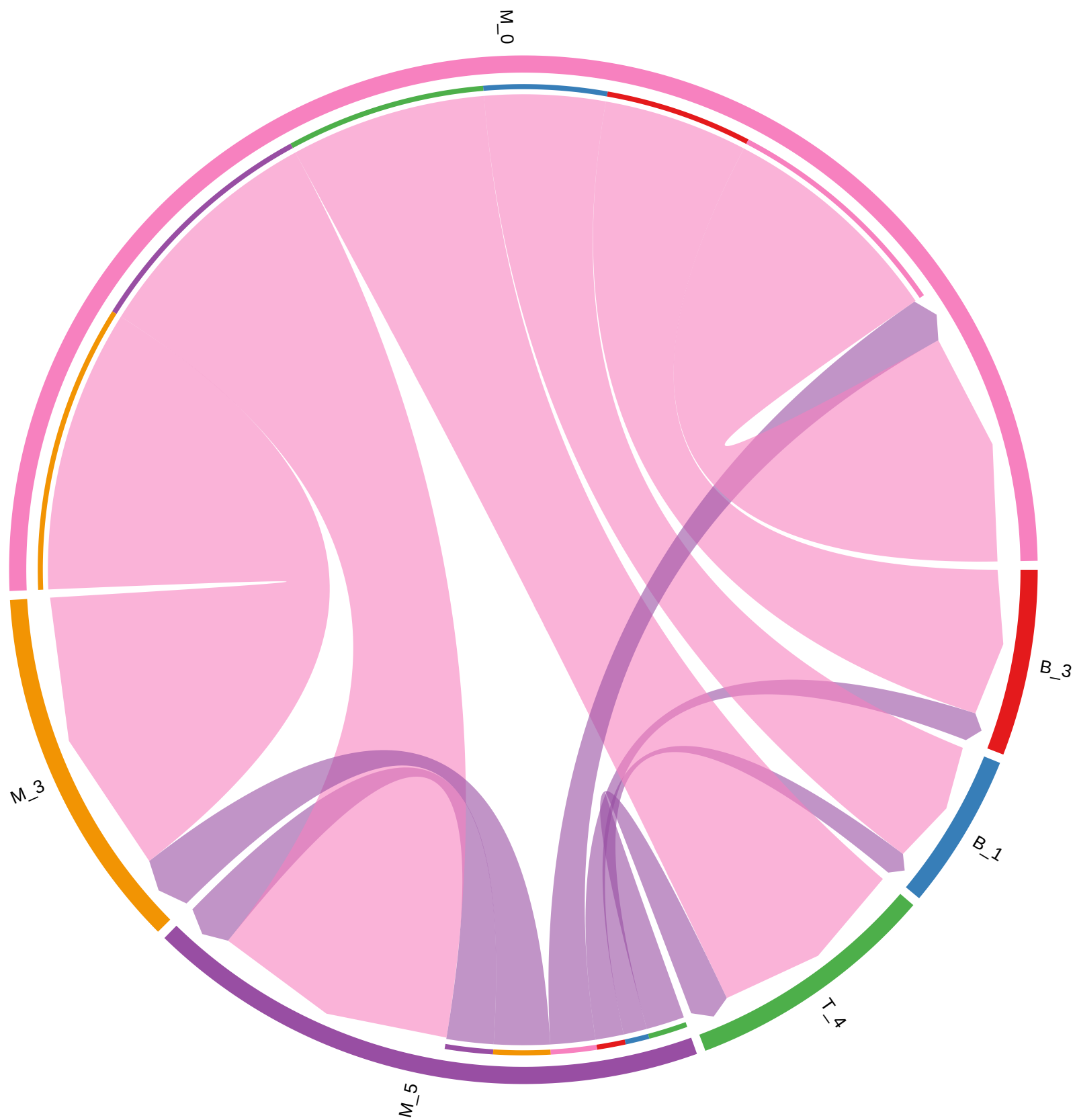
SIRP signaling pathway network
