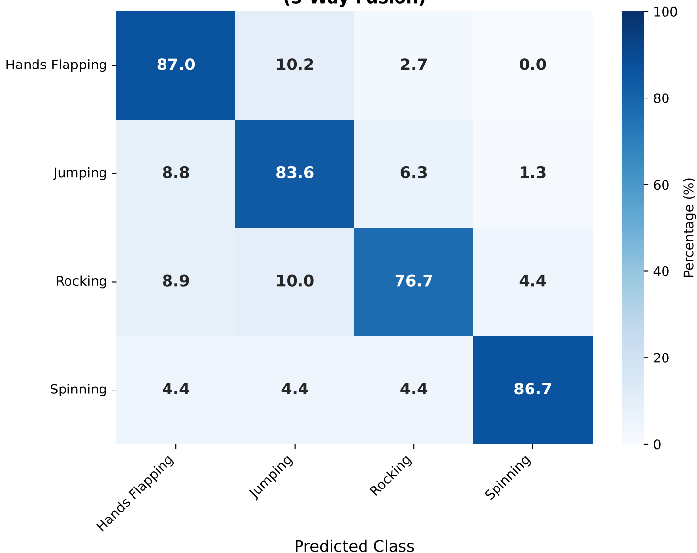
4-Class Classification Confusion Matrix (3-Way Fusion)
