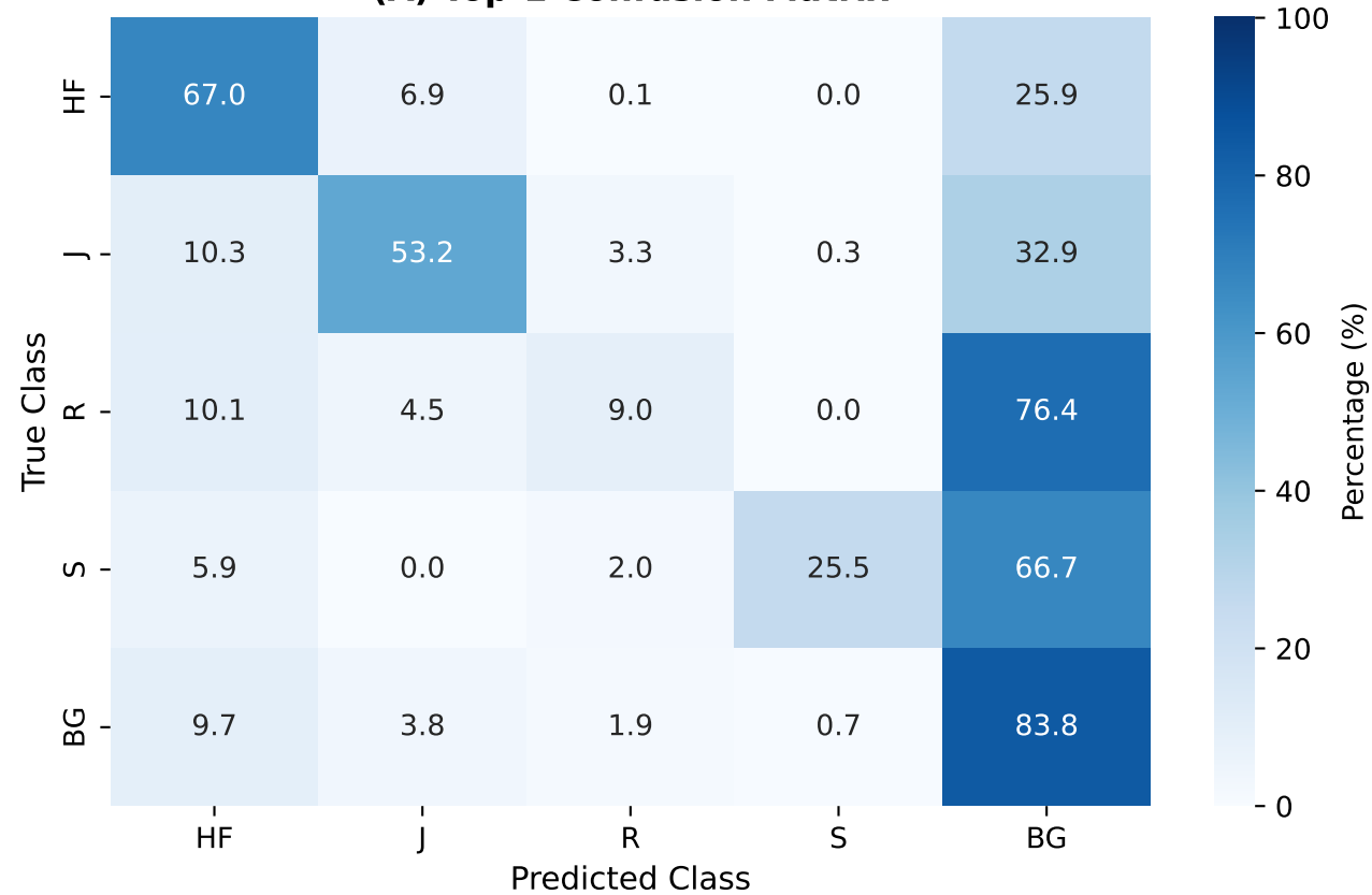
(A) Top-1 Confusion Matrix
