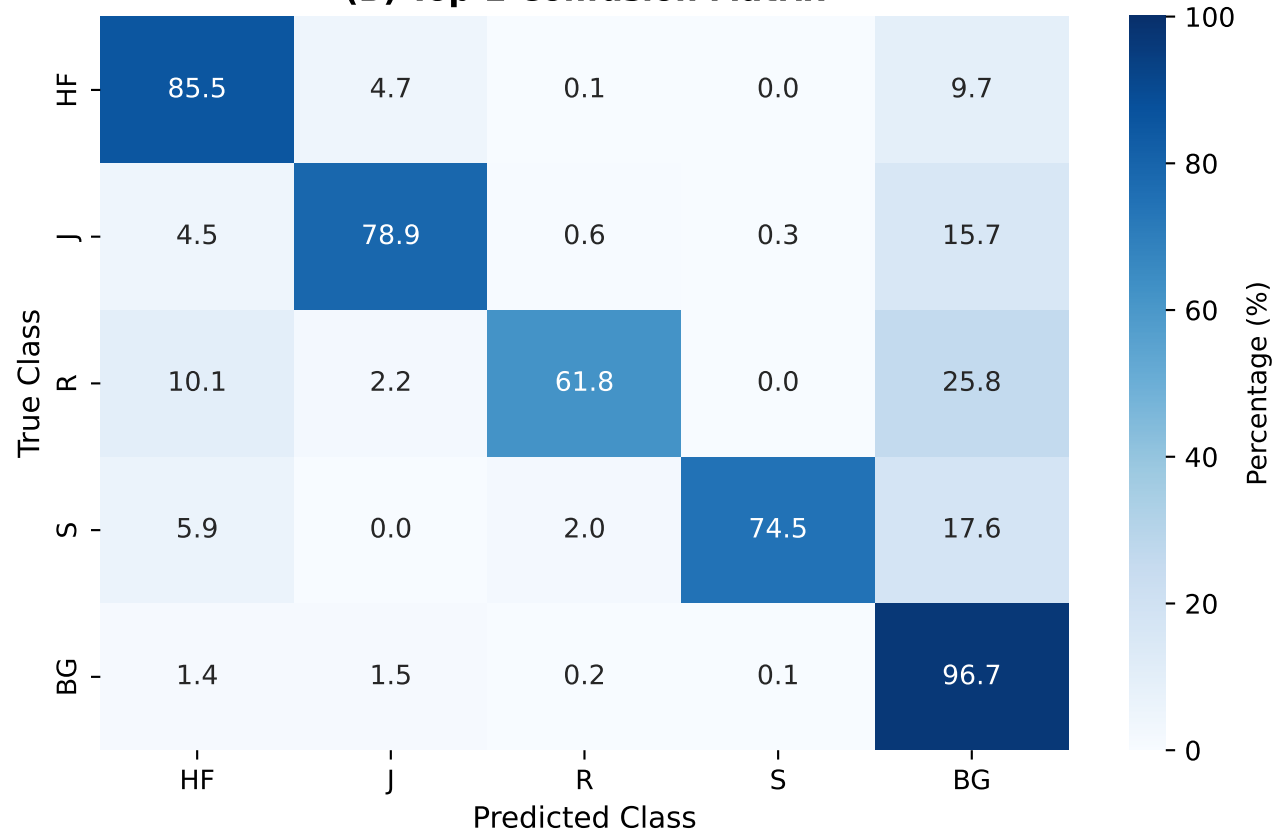
(B) Top-2 Confusion Matrix
