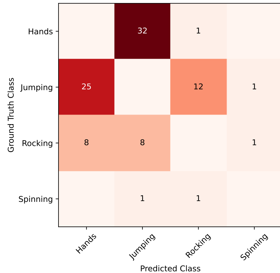
Class Confusion Matrix (Localized but Misclassified)
