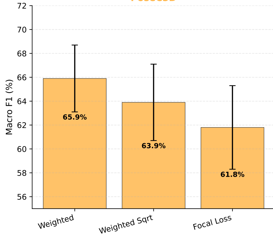
PoseC3D
