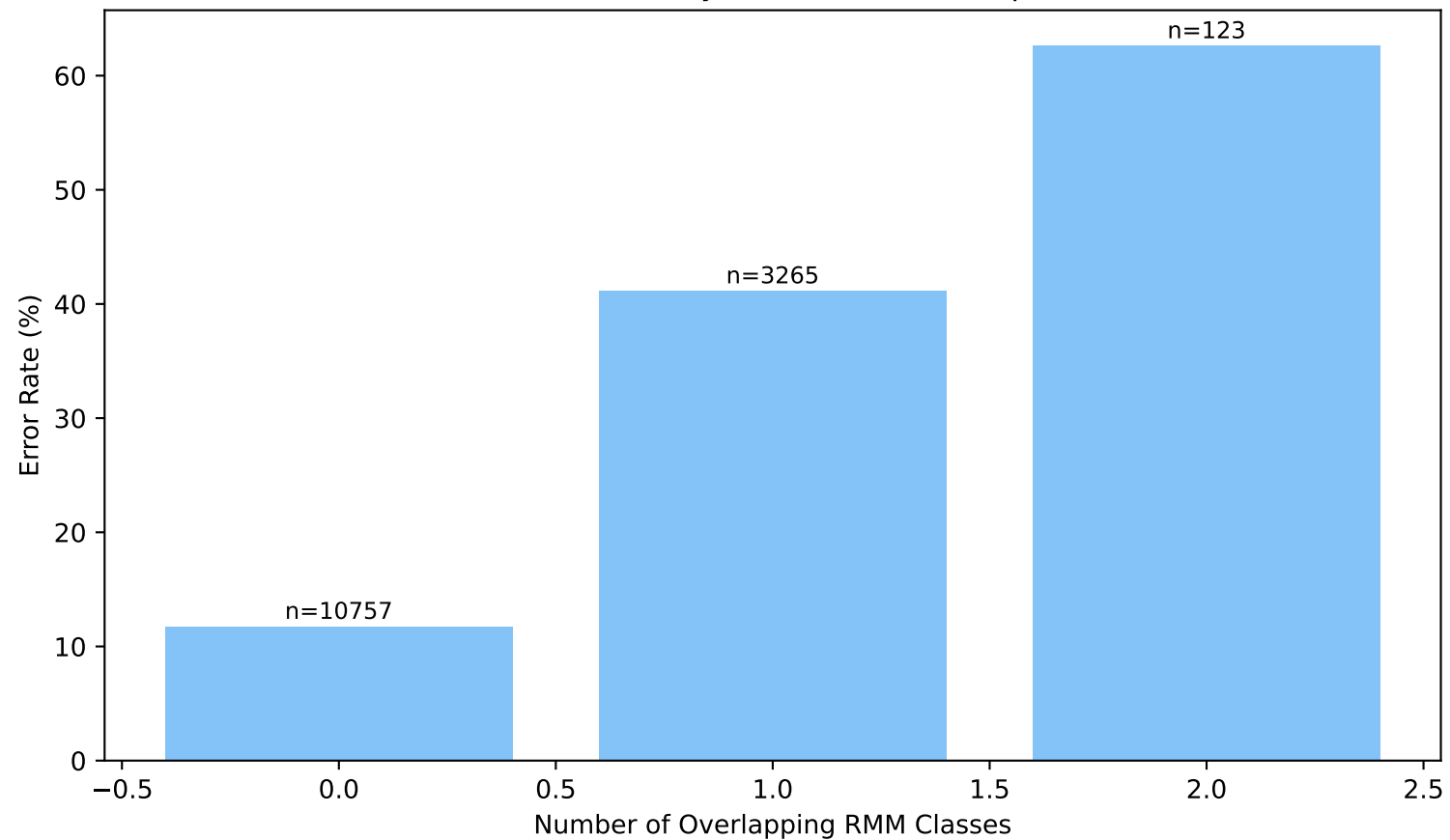
Error Rate by Multi-Label Overlap
