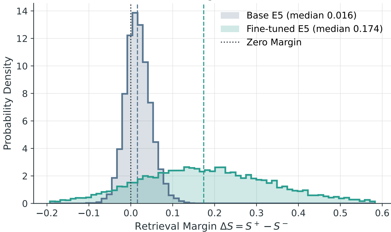
Retrieval Margin Distribution
