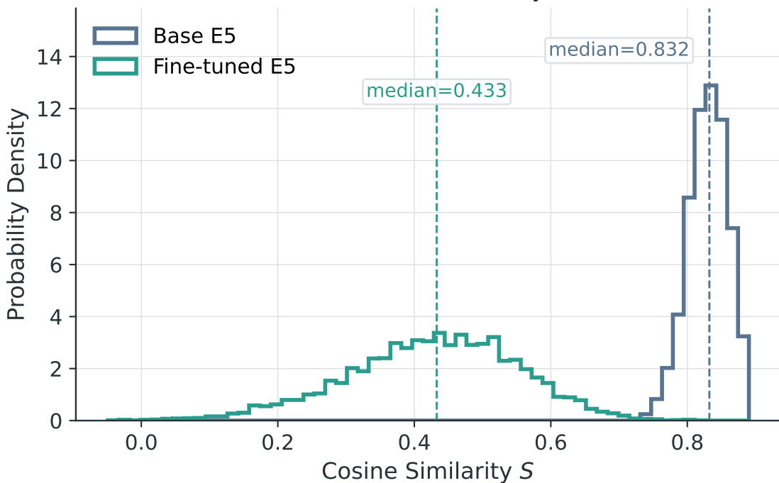
Correct Chunk Similarity S^+
