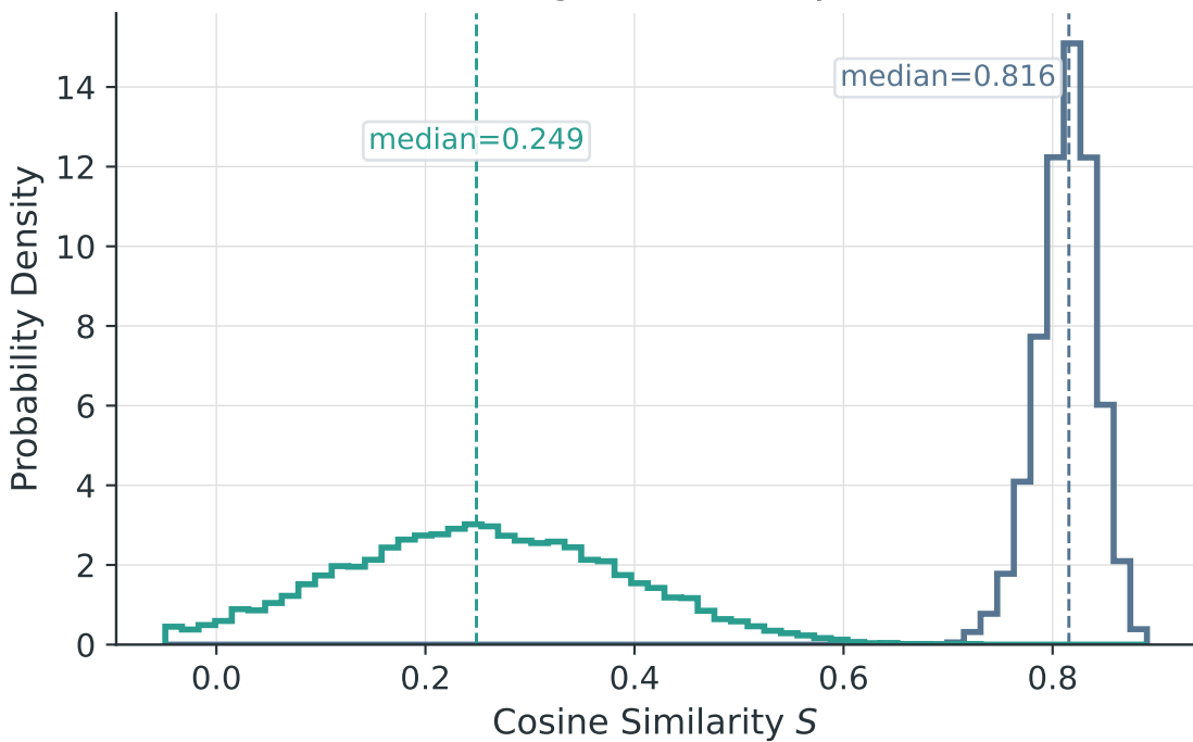
Hard Negative Similarity S^-
