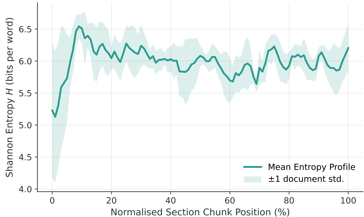
Mean Entropy Profile Across Documents
