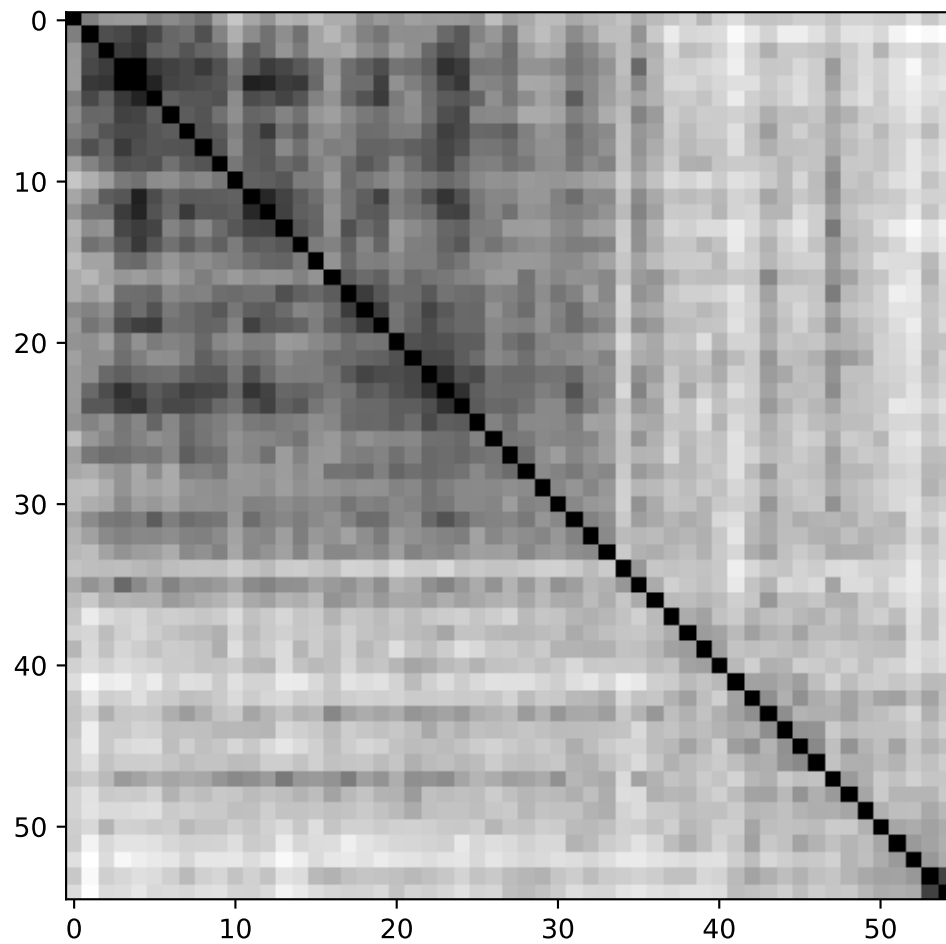
Permutation
