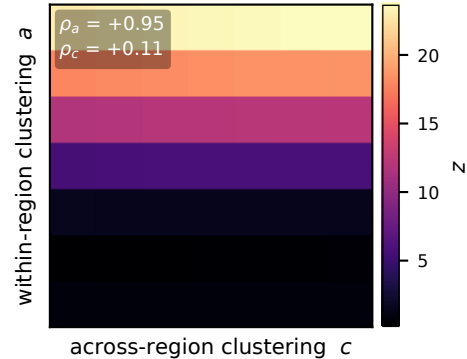
clustering in neuron space
