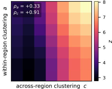
clustering in region space (Procrustes)
