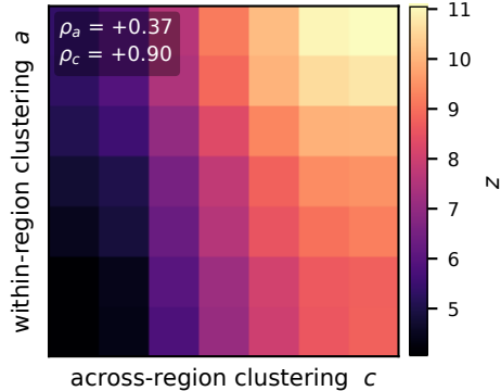
clustering in region space (DECODING)
