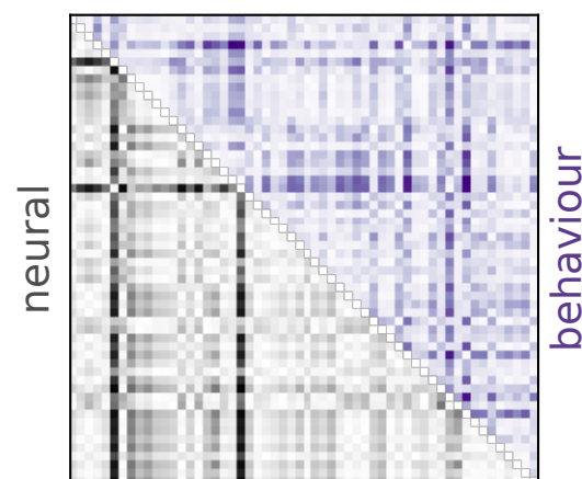
g pairwise distances
