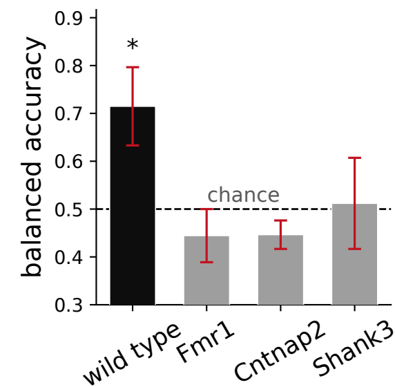
d genotype decoding
