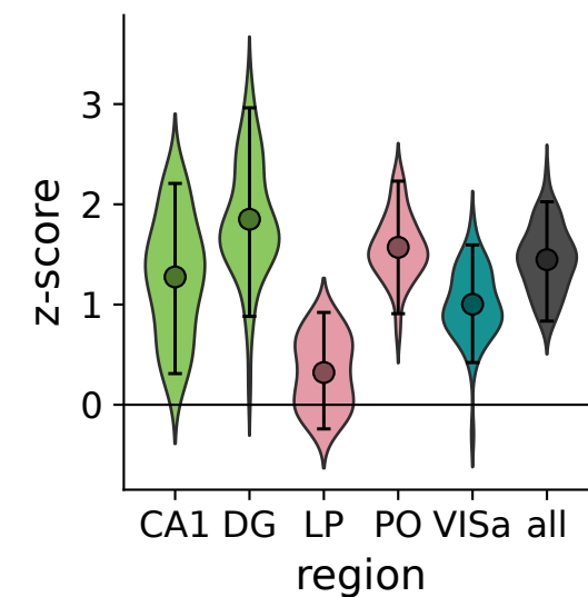
i behaviour-neural correlation (shuffle corrected)
