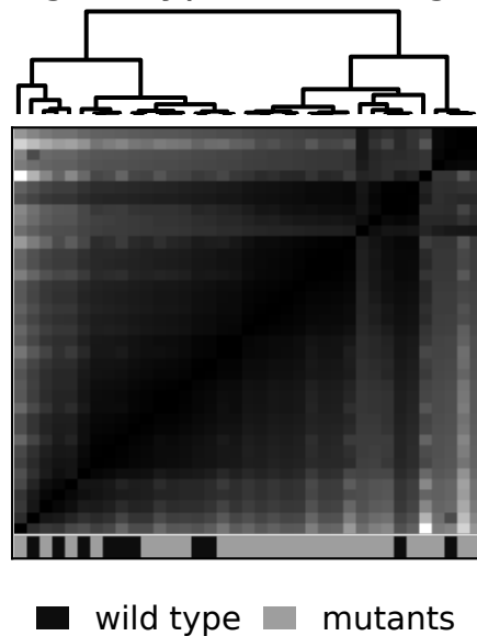
b genotype clustering
