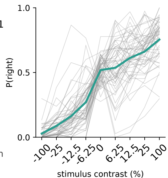
f behaviour, 56 mice
