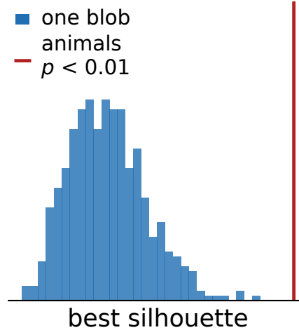
c all genotypes (n = 36)
