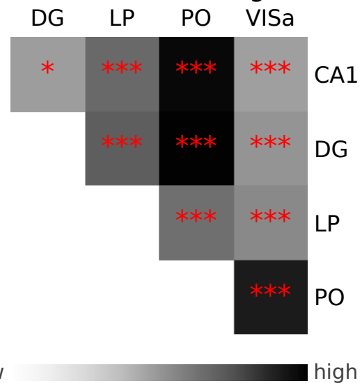
e distances across regions
