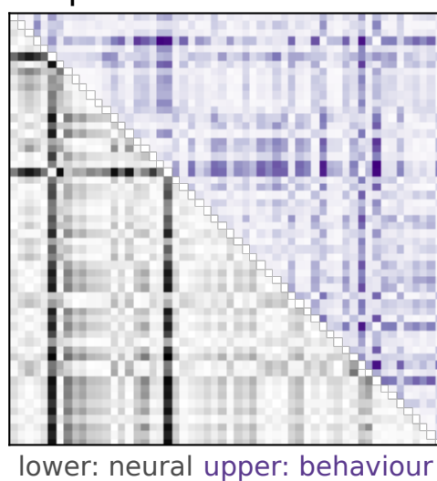
d pairwise distances
