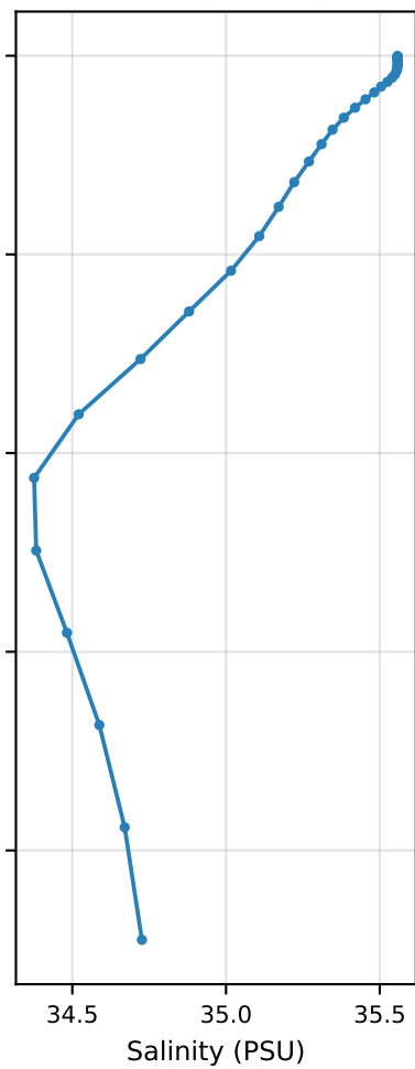
Mean Salinity (PSU) profile
