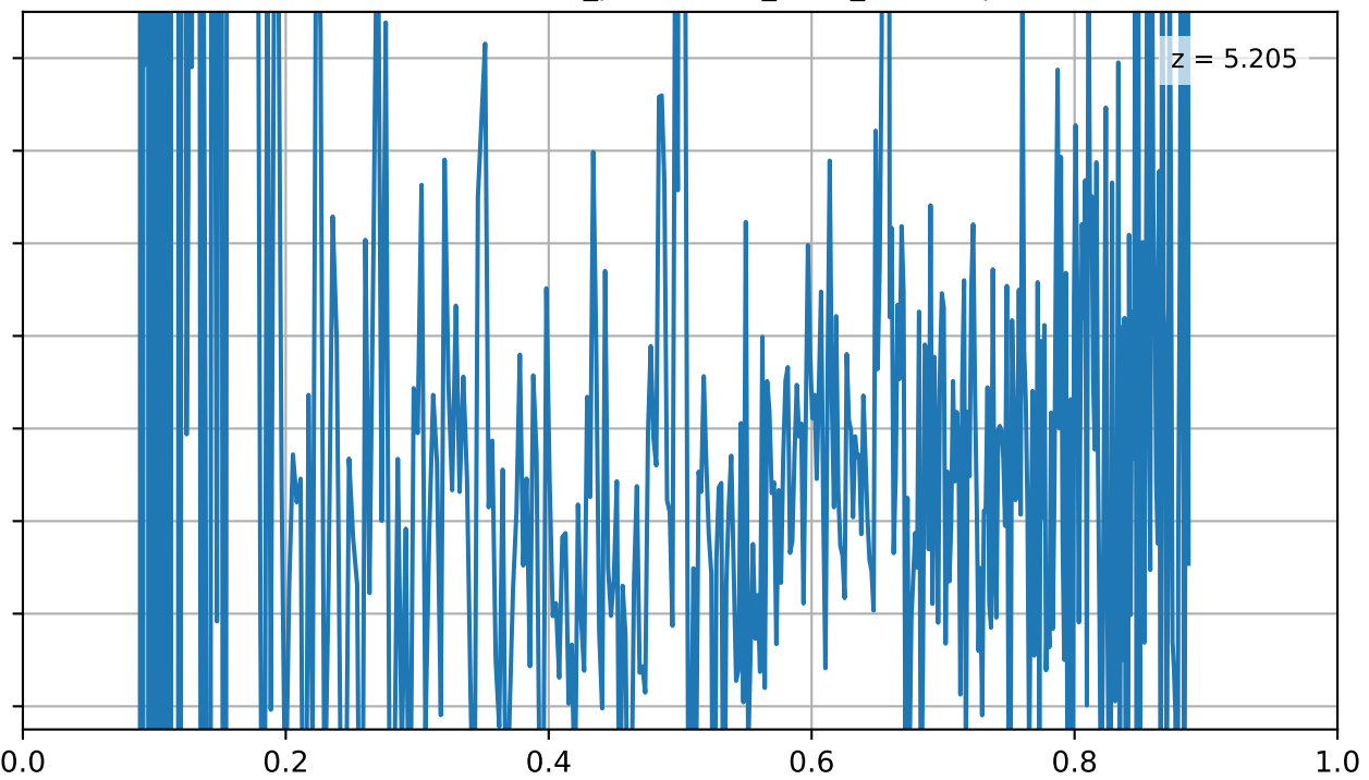
cosmos-transients-v4_prism-clear_6585_65449.spec.fits
