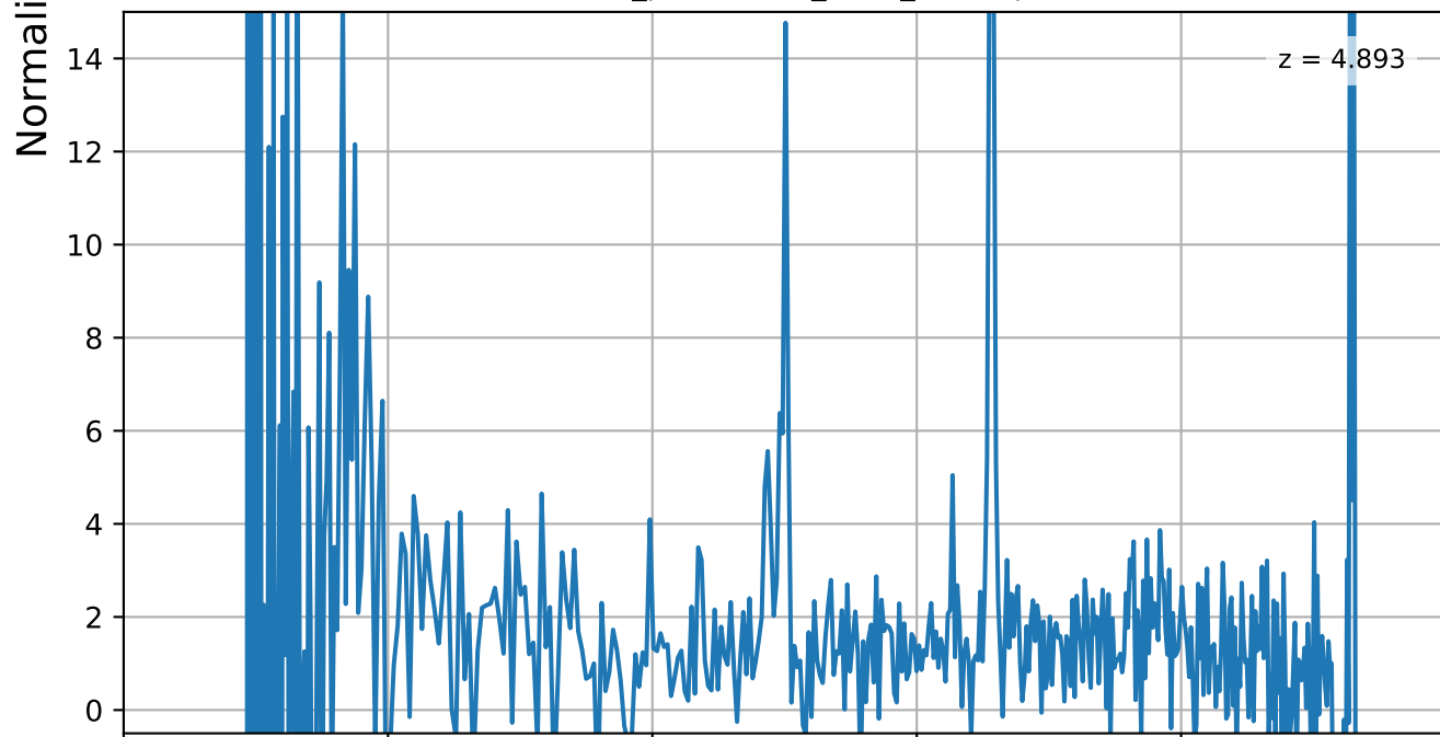
cosmos-transients-v4_prism-clear_6585_61234.spec.fits
