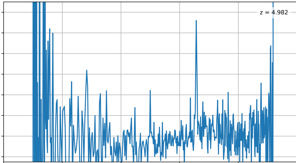
uncover-61-v4_prism-clear_2561_21547.spec.fits
