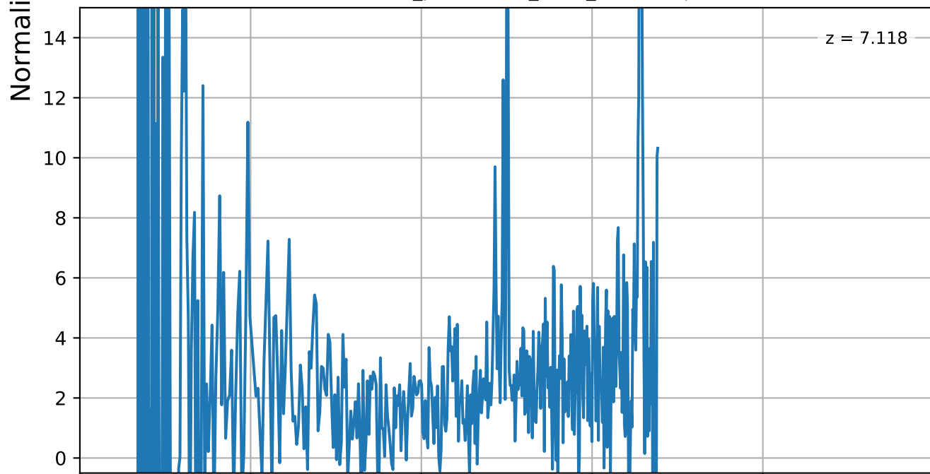
uncover-61-v4_prism-clear_2561_24968.spec.fits
