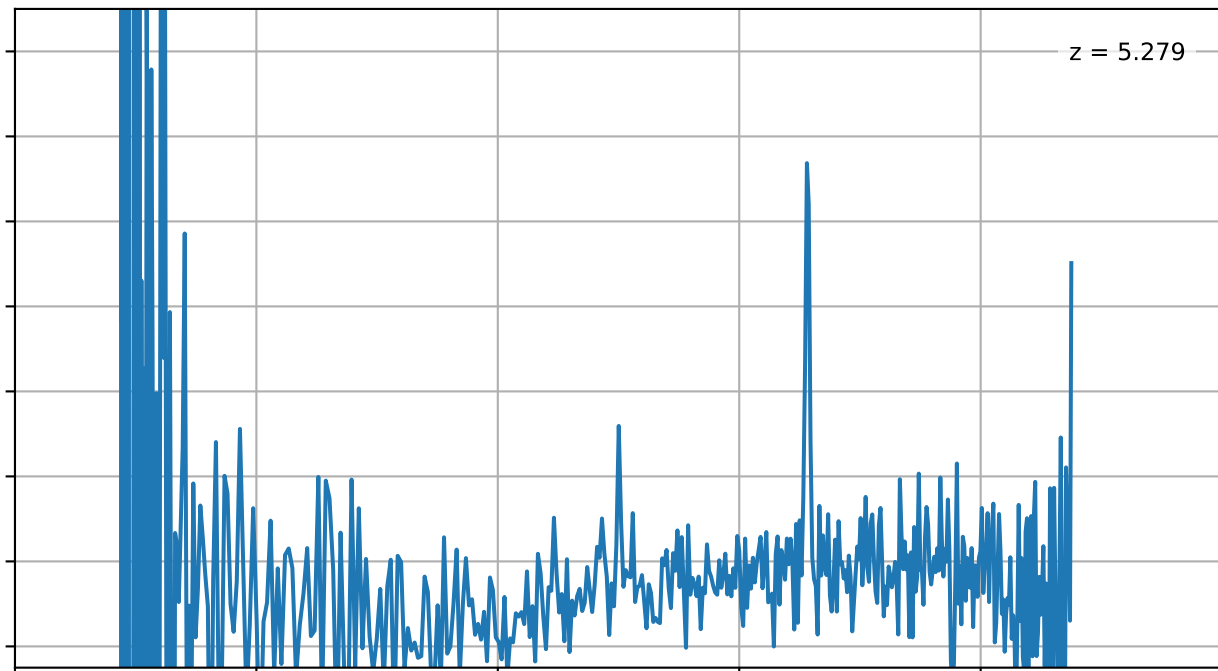
rubies-uds43-v4_prism-clear_4233_40800.spec.fits
