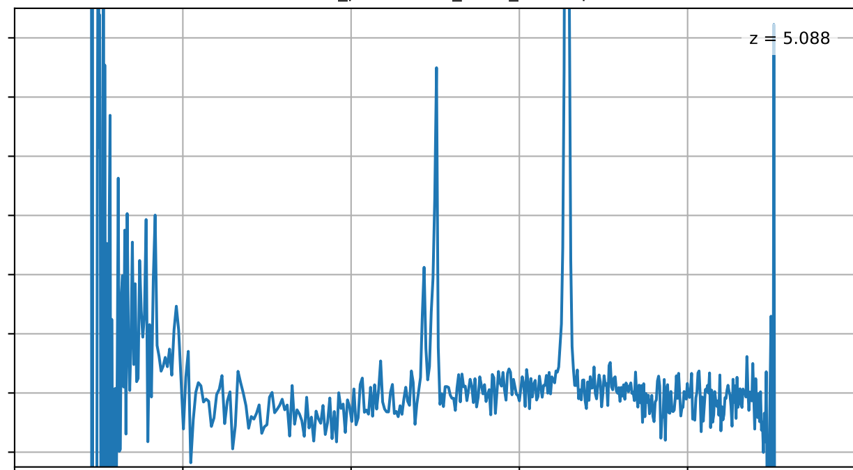
ceers-ddt-v4_prism-clear_2750_1768.spec.fits
