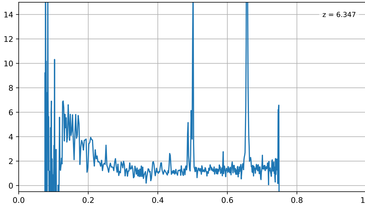
uncover-61-v4_prism-clear_2561_24968.spec.fits
