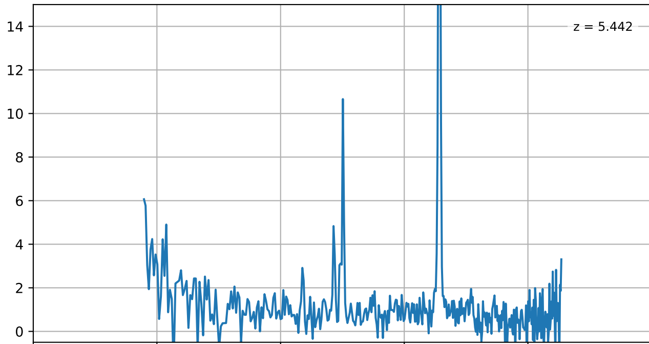
rubies-uds33-v4_prism-clear_4233_29813.spec.fits
