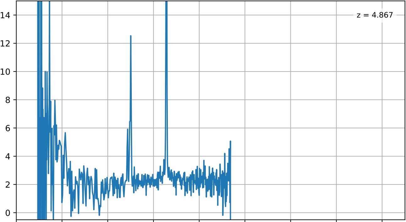
uncover-v4_prism-clear_2561_49702.spec.fits
