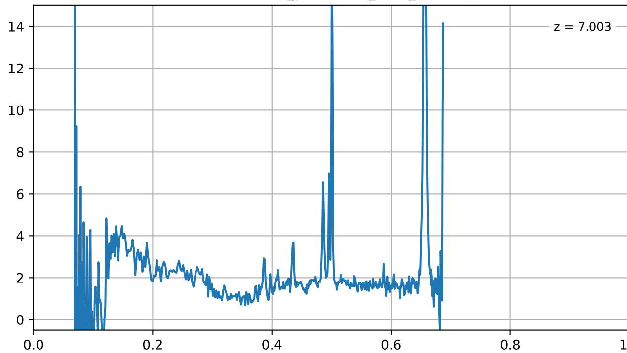
cosmos-transients-v4_prism-clear_6585_61234.spec.fits
