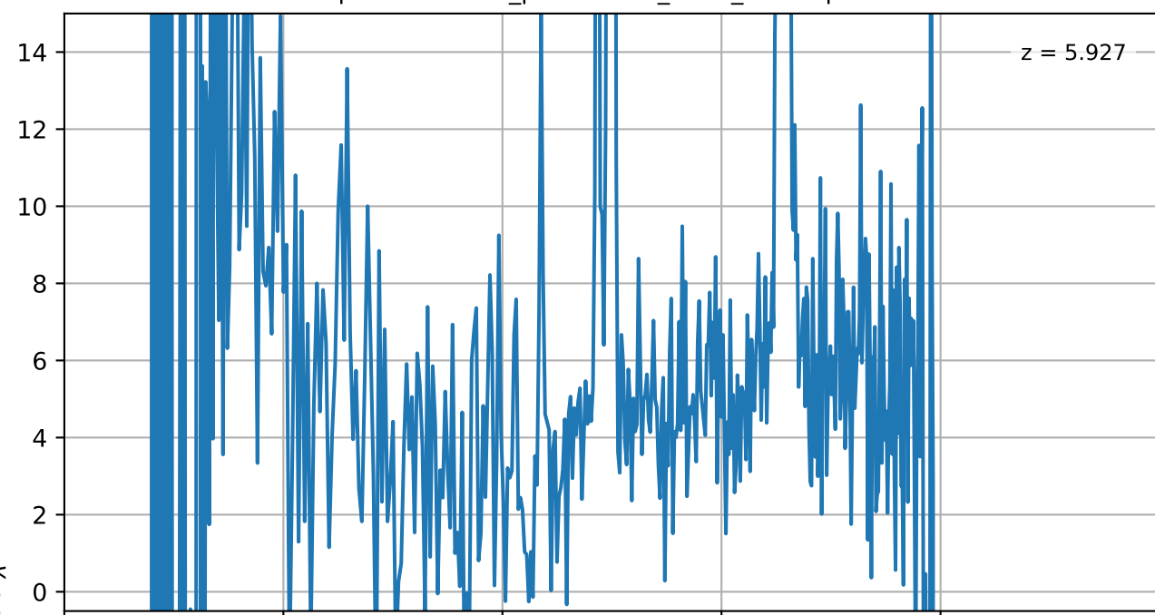
capers-egs49-v4_prism-clear_6368_11585.spec.fits
