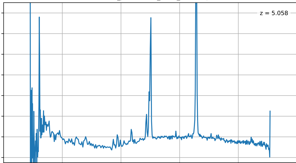
uncover-61-v4_prism-clear_2561_27114.spec.fits
