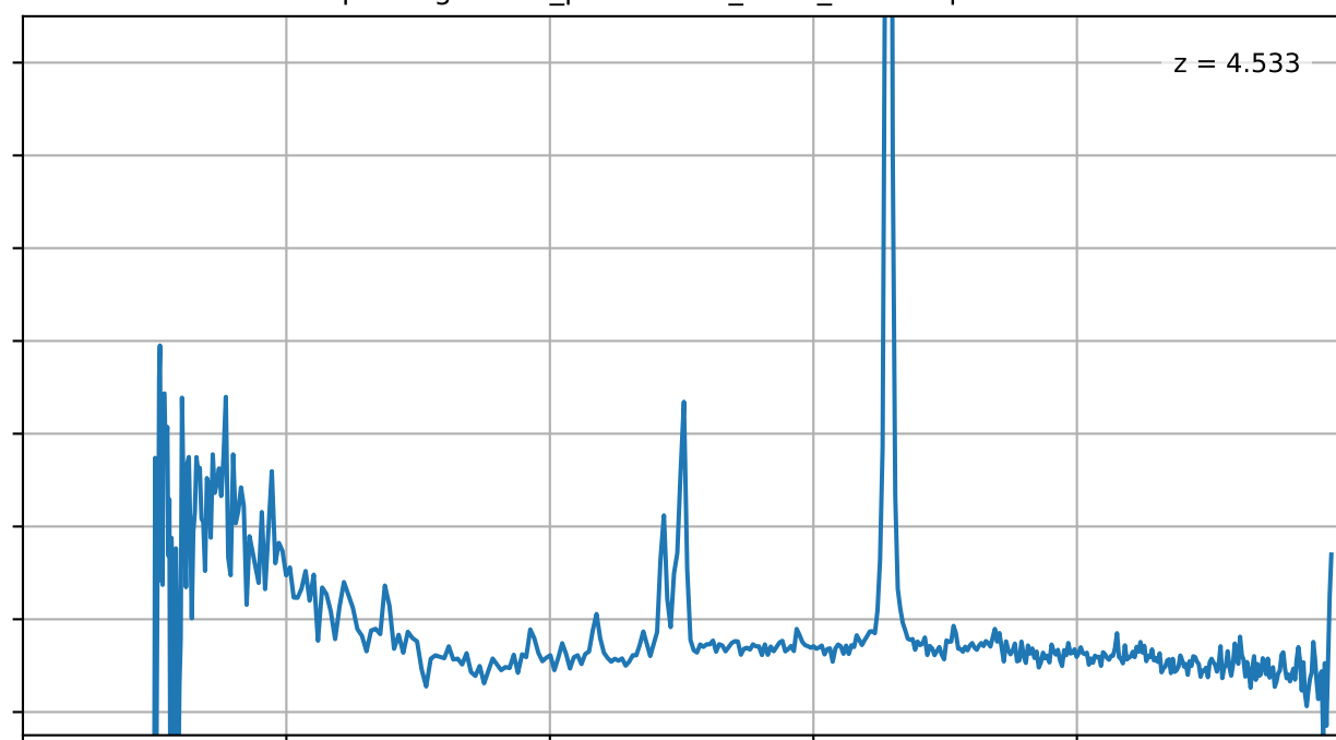
capers-egs49-v4_prism-clear_6368_8752.spec.fits
