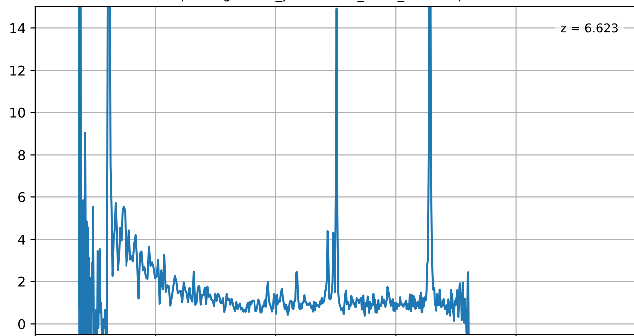
capers-egs53-v4_prism-clear_6368_10108.spec.fits
