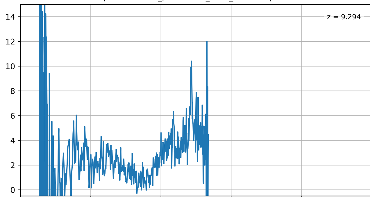
capers-cos19-v4_prism-clear_6368_4771.spec.fits
