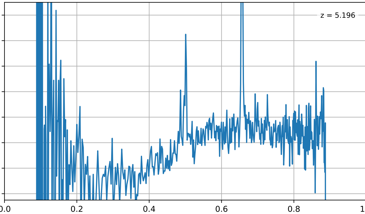
uncover-61-v4_prism-clear_2561_27114.spec.fits
