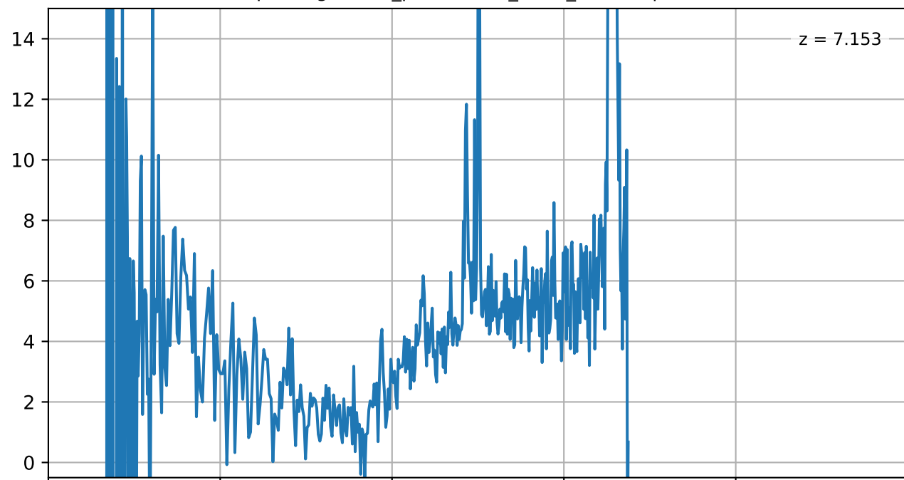
capers-udsp2-v4_prism-clear_6368_10997.spec.fits
