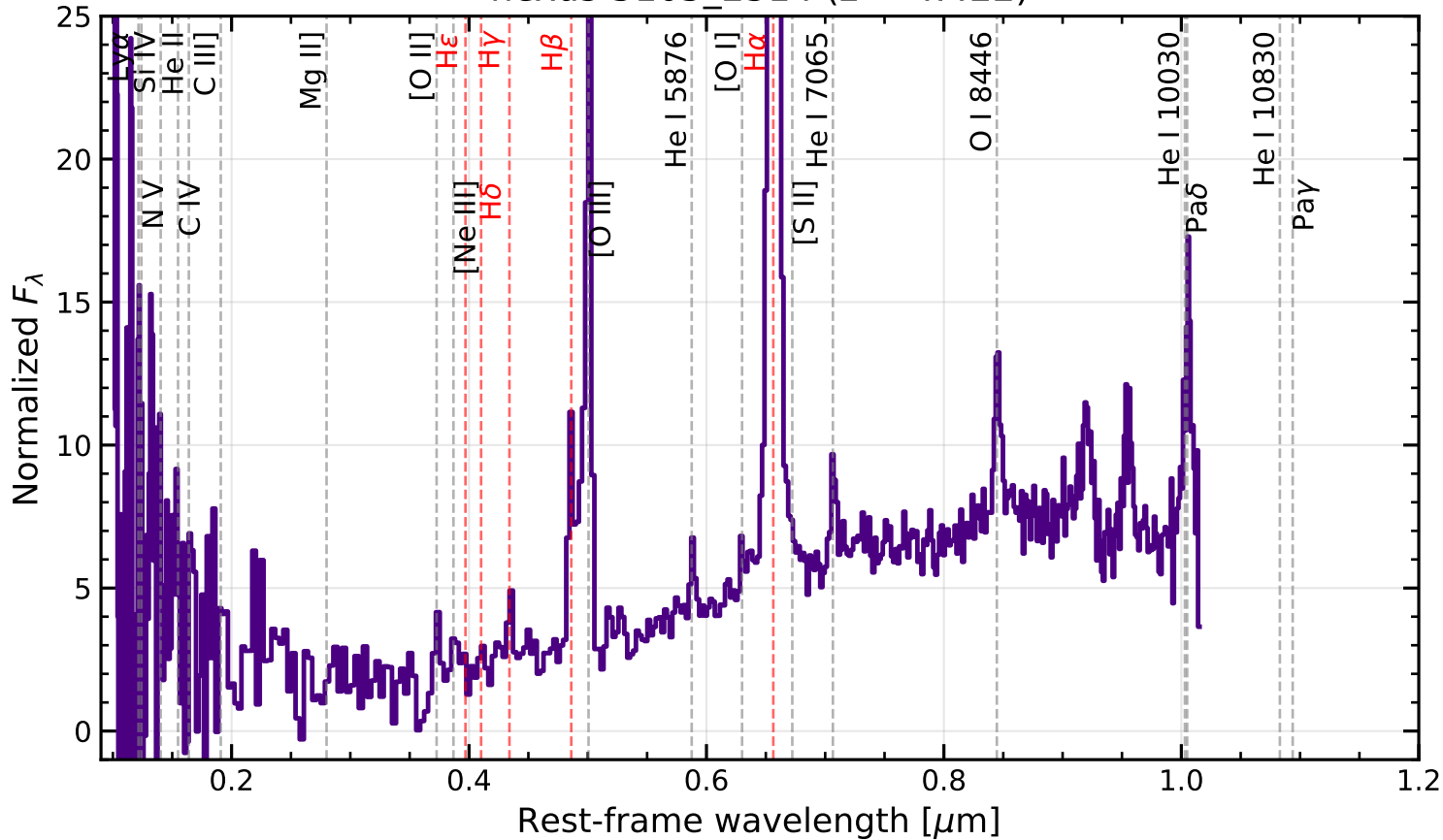
nexus-5105_2314 ( z = 4.422 )
