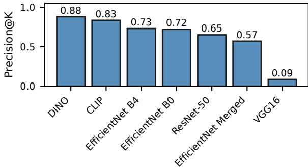
Image Retrieval: Precision@K by Model
