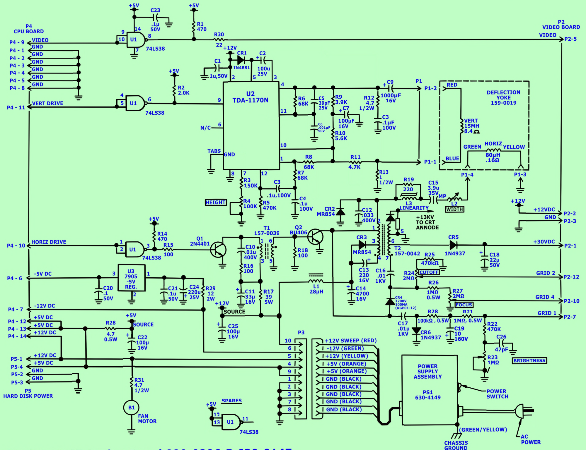
Macintosh SE Analog Board 820-0206-B 630-0147
