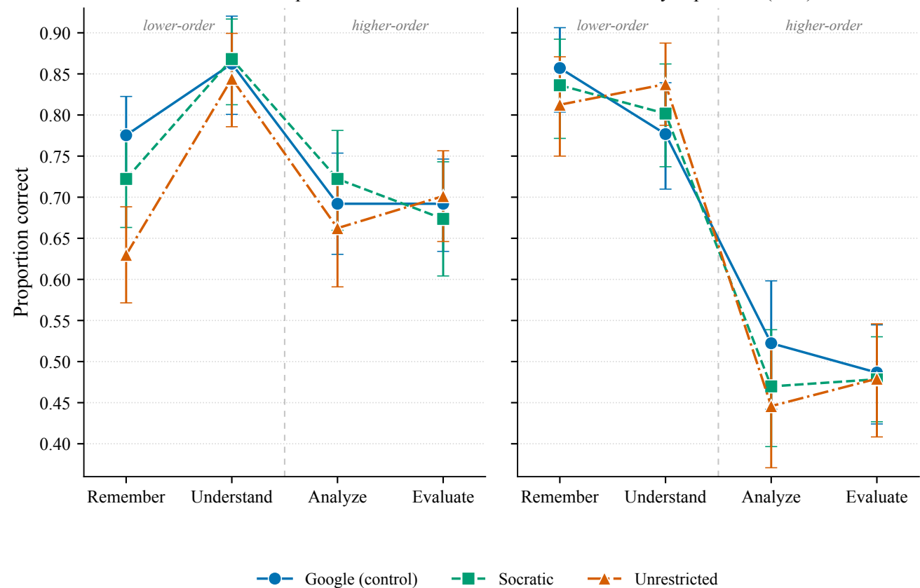
Immediate post-test
