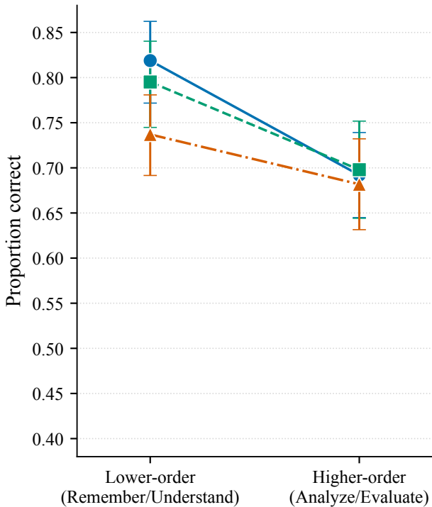
Immediate post-test
