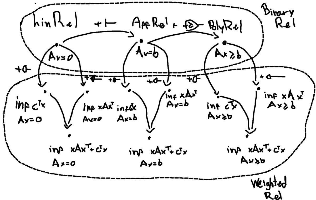
Figura 1.1 – This image represent the category of subcategories of \text{Rel} ; We circle two class of subcategories, namely those that are contained in the Binary Relations categories and those embed in Weighted Relations category. Observe how morphism between objects (class of relations) are the addition of a single generator (along with some axioms), and that there are particular generators which are essential binary relations (those that are horizontal) that keeps objects in the subclass of binary relations, but there are others (the vertical morphisms), that resembles an output or measurement, that lift the relations to those on the Weighted Relations class
