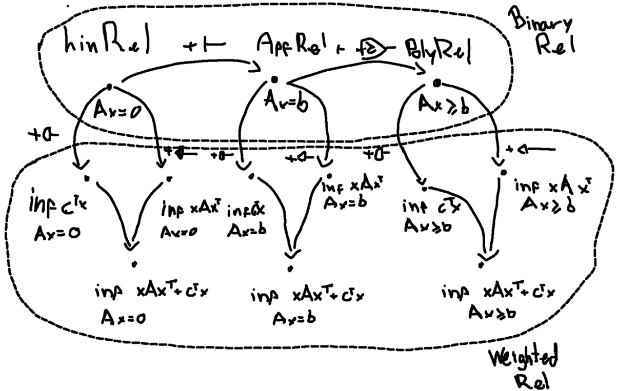
Figure 1.1 – This image represents the category of subcategories of \mathbf{Rel} . We circle two classes of subcategories: those contained in the Binary Relations category, and those embedded in the Weighted Relations category. Morphisms between objects (classes of relations) correspond to the addition of a single generator, together with some axioms. The horizontal morphisms add generators that are themselves binary relations, keeping the object in the subclass of binary relations. The vertical morphisms, by contrast, add a generator that resembles an output or measurement, lifting the relation into the Weighted Relations class.
