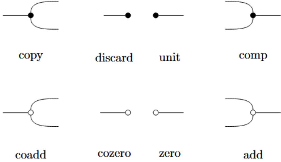
Figure 2.1 – Frobenius additive(black) and co-additive(white) structure
