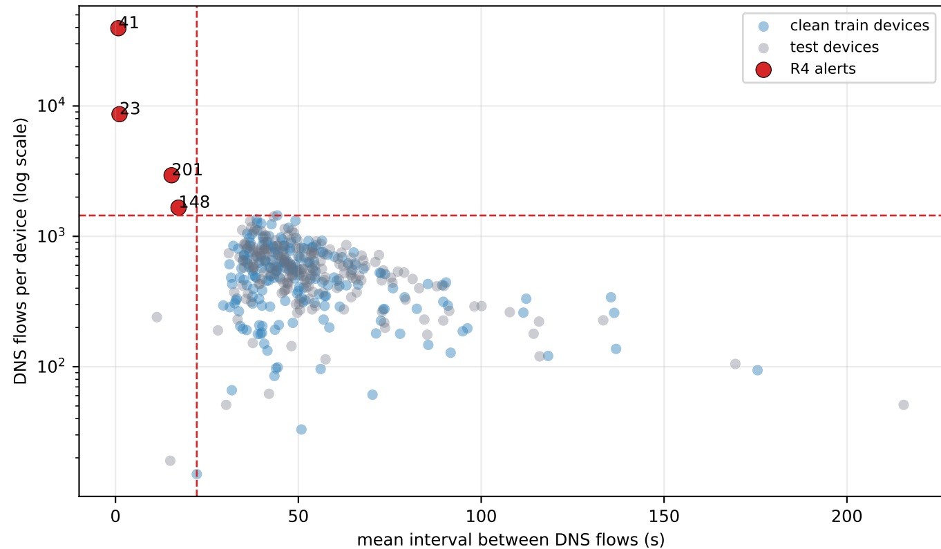
DNS C&C: high flow count plus short polling interval
