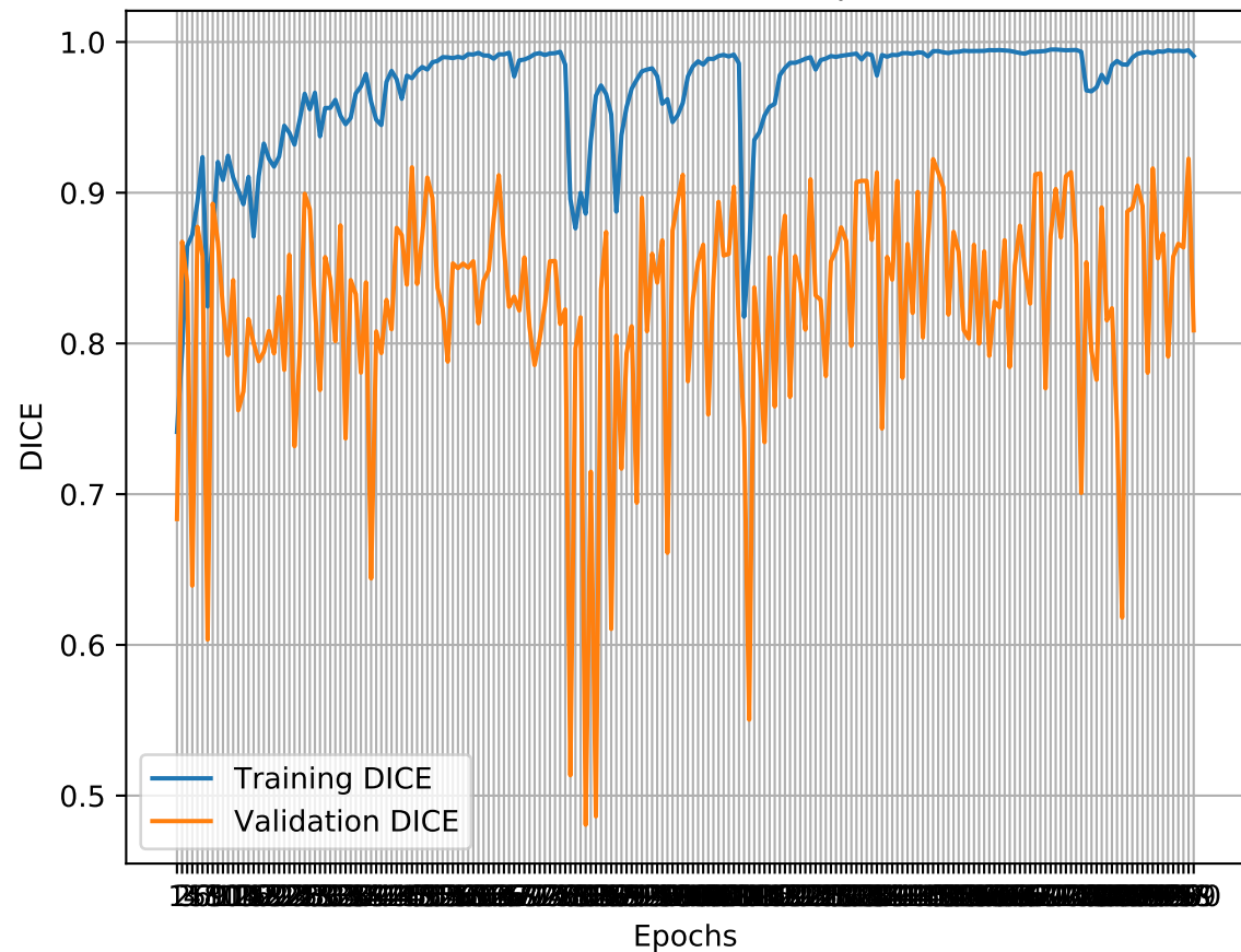
DICE Coefficient over epochs
