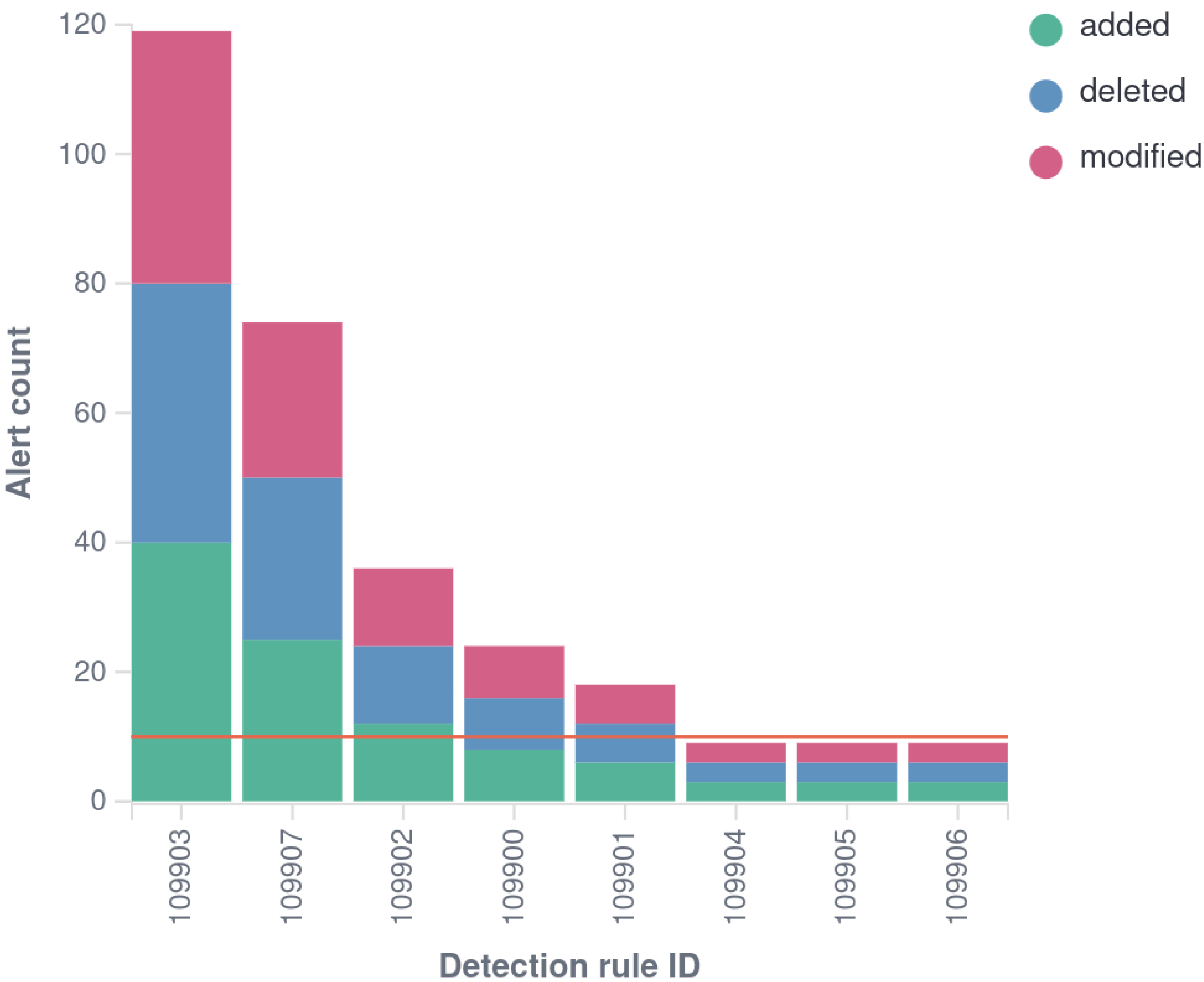
FIM — Alerts by Detection Rule and Event Type
