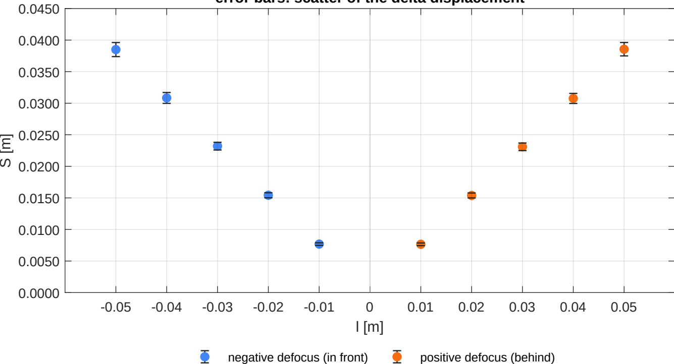
Sensitivity for f = 200 mm (slider-sweep) error bars: scatter of the delta displacement
