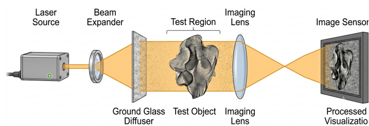
Figure 3.7: Illustration of a SBOS setup using ground-glass-diffused laser speckles, similar to Michalski's setup [32]
