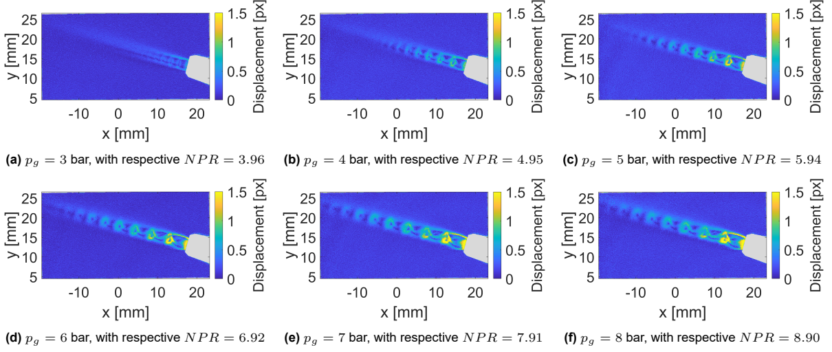
Figure 6.7: SBOS results for a compressible jet. Displacement magnitude fields obtained through cross correlation for air tap gauge pressures from 3 bar to 8 bar with a step of 1 bar. All fields share the same colour scale and masked vectors are shown in grey
