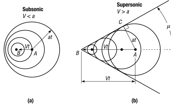
Figure 2.1: Propagation of information by an object moving at (a) subsonic speeds and (b) supersonic speeds, credit to Anderson [27]
