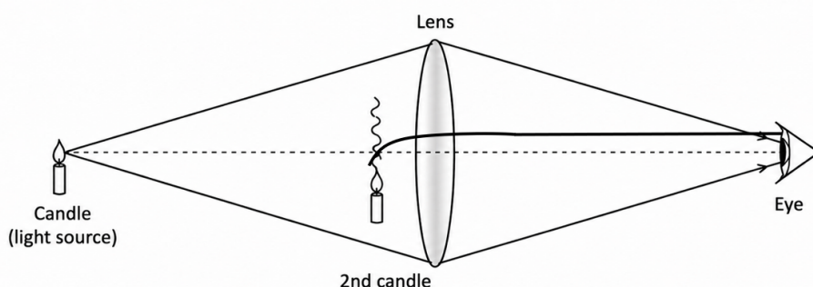
Figure 3.1: Hooke's shadowgraphy setup, credit Settles [46]
