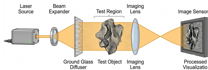
Figure 3.7: Illustration of a SBOS setup using ground-glass-diffused laser speckles, similar to Michalski's setup [33]
