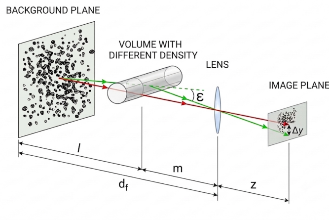
Figure 3.4: BOS setup, credit to Raffel [41]
