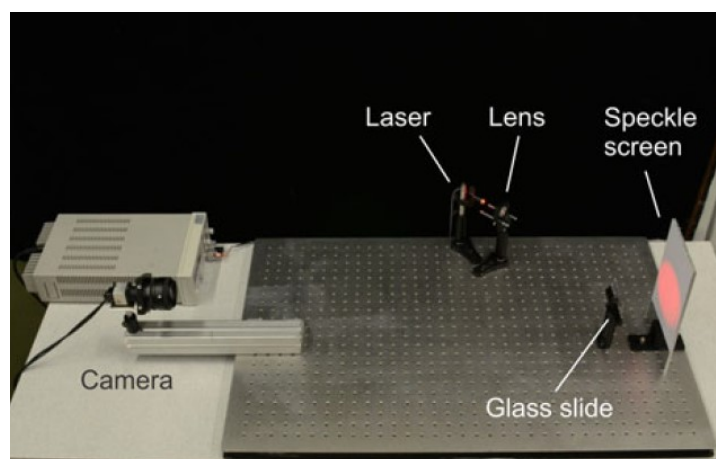
Figure 3.6: Experimental SBOS setup (single pass) used by Meier and Rösger [32]
