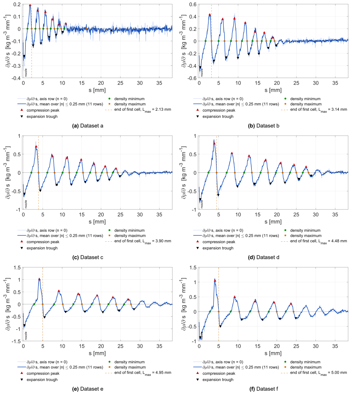
Figure 6.9: Centerline density gradient in the s direction for datasets a to f, obtained assuming a planar field. The light blue line is the gradient at the axis row n = 0 and the dark blue line its mean over |n| \leq 0.25 mm. The markers indicate the compression peaks, expansion troughs, density minima and density maxima detected along the centerline, and the dashed line marks the end of the first shock cell
