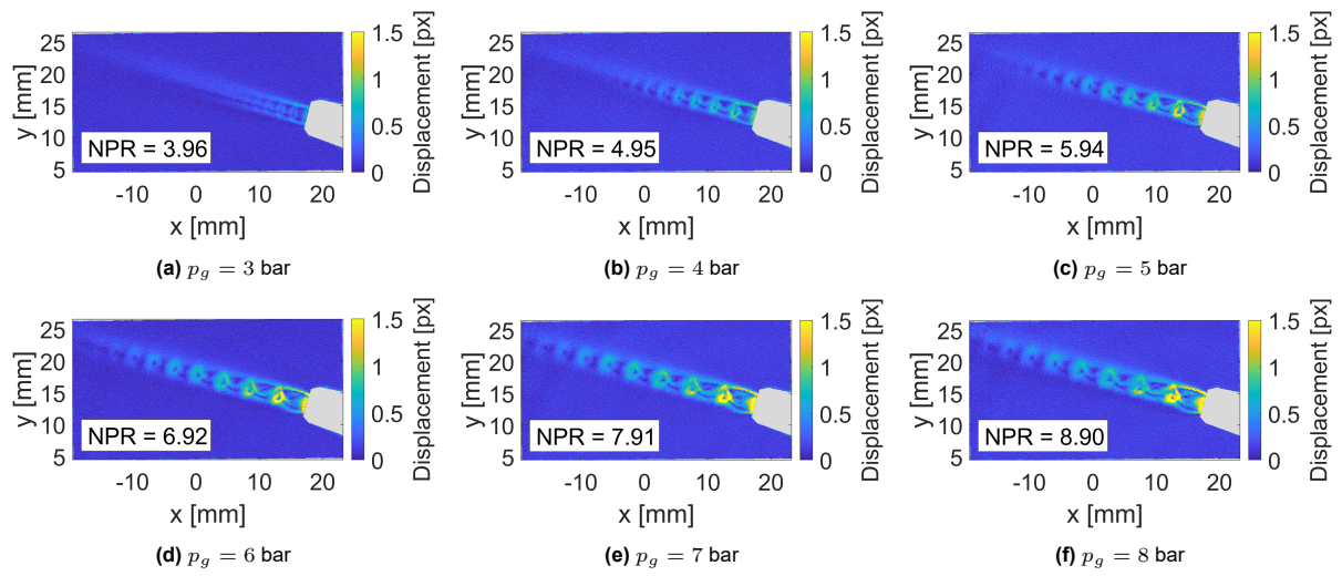
Figure 6.7: Displacement magnitude fields of the compressible jet obtained through cross correlation for gauge pressures from 3 bar to 8 bar with a step of 1 bar. The NPR of each case is shown in its legend. All fields share the same colour scale and masked vectors are shown in grey
