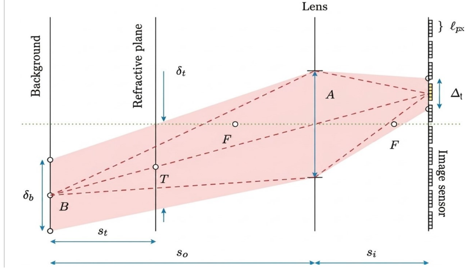
Figure 3.5: Diagram of the cone of light that reaches a length in the sensor \Delta_t , this image was used by Gojani et al. to derive his equation for spatial resolution. Credit to Gojani et al. [13]
