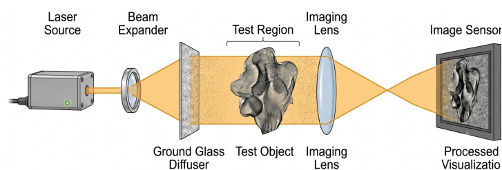
Figure 3.7: Illustration of a SBOS setup using ground-glass-diffused laser speckles, similar to Michalski's setup [31]
