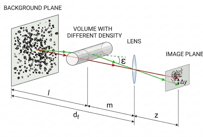
Figure 3.4: BOS setup, credit to Raffel [38]
