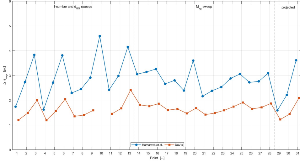
Figure 6.2: Average speckle size of every point of Table 6.7, computed with the autocorrelation method of Hamarová et al. [17] and with the DaVis function. The dashed lines separate the f_{\#} and d_{GG} sweeps, the magnification sweep and the projected speckle points. DaVis returned no value for point 10
