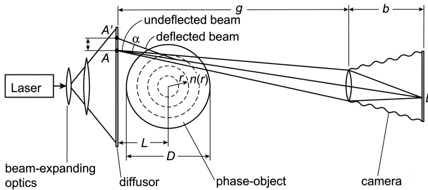
Figure 3.3: Laser-speckled Interferometry setup, credit to Köpf [28]
