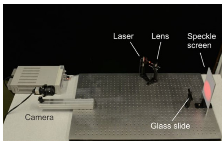
Figure 3.6: Experimental SBOS setup (single pass) used by Meier and Rösger [30]
