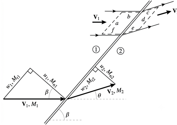
Figure 2.2: Oblique shock geometry, credit to Anderson [25]
