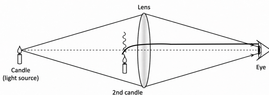
Figure 3.1: Hooke's shadowgraphy setup, credit Settles [43]
