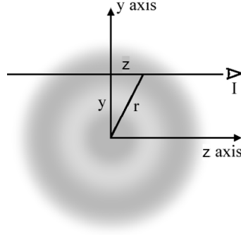
Figure 2.7: Diagram of the geometry of an axisymmetric body being seen by an observer in I. If the body, in grey, is described by a function f(r) , the observer will see its projection F(y) , which is its Abel transform
