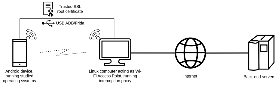
Fig. 1. Measurement setup. The Android device running the investigated operating systems is configured to access the Internet using Wi-Fi. The access point is hosted on a Linux computer, running traffic interception and capture software. A custom system certificate is installed on the phone using root access. A USB connection is used for ADB/Frida communication.
