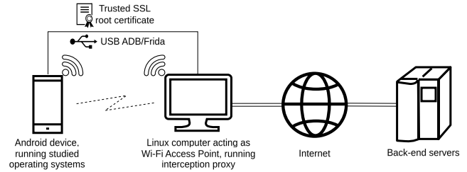
Figure 1: Measurement setup. The Android device running the investigated operating systems is configured to access the Internet using Wi-Fi. The access point is hosted on a Linux computer, running traffic interception and capture software. A custom system certificate is installed on the phone using root access. A USB connection is used for ADB/Frida communication.
