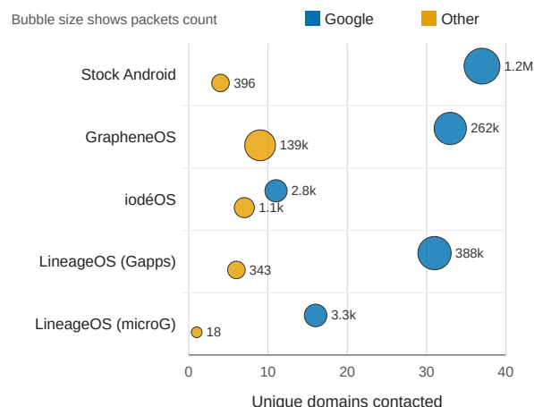
Figure 3: Domains contacted in Scenario A1 aggregated for all tasks, grouped by operating system and by Google-related and other endpoints. Bubble size represents the total number of packets exchanged with each group.
