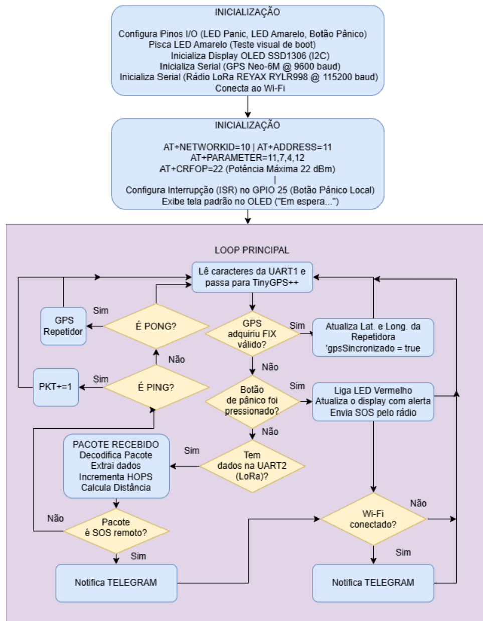
Figura 11 – Fluxograma do Firmware
