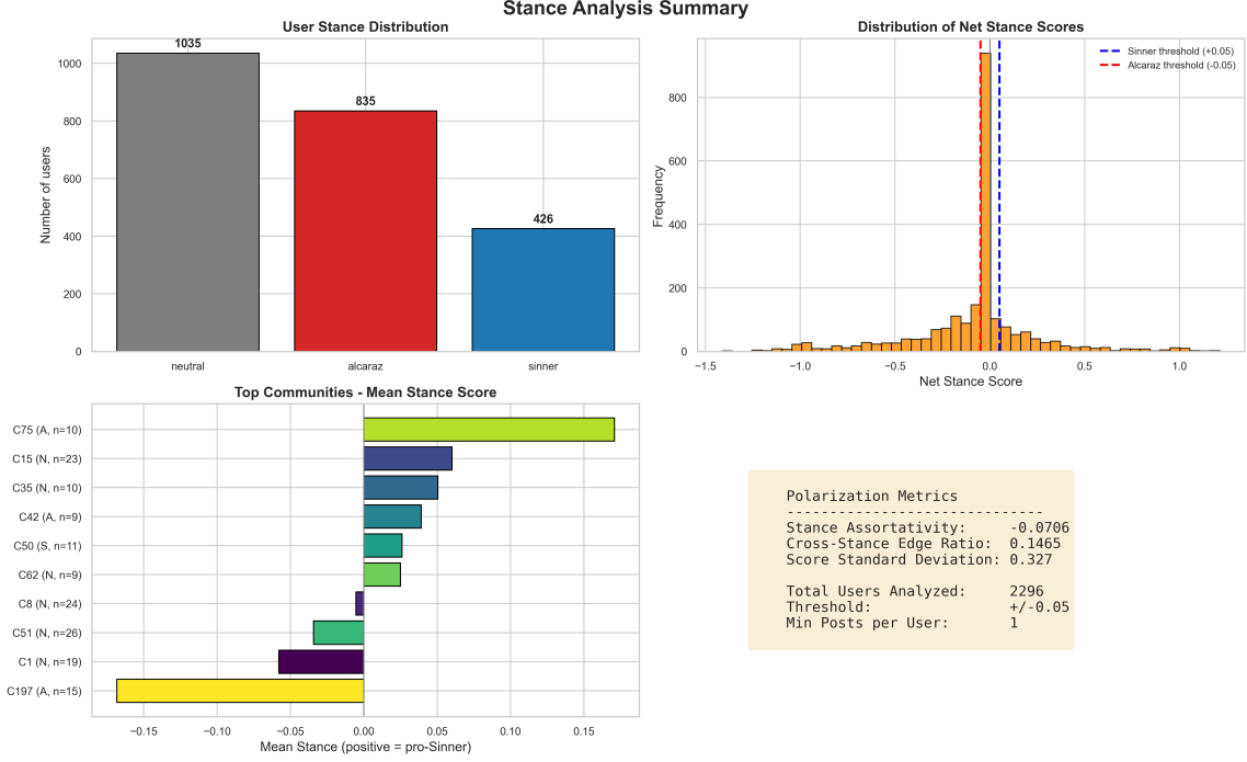
Figure 8: Stance analysis summary. Top-left: user stance counts (neutral 1035, Alcaraz 835, Sinner 426). Top-right: net-stance score histogram with \pm 0.05 thresholds. Bottom-left: mean stance of top communities. Bottom-right: polarisation metrics (assortativity -0.071 , cross-stance edge ratio 0.147 , score SD 0.327 ).
