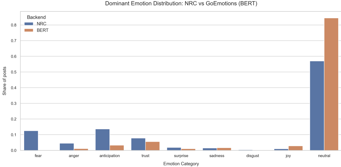
Figure 6: Dominant emotion distribution: NRC lexicon vs. GoEmotions (BERT). The neural backend labels more posts neutral; the lexicon assigns more anticipation/fear/trust.
