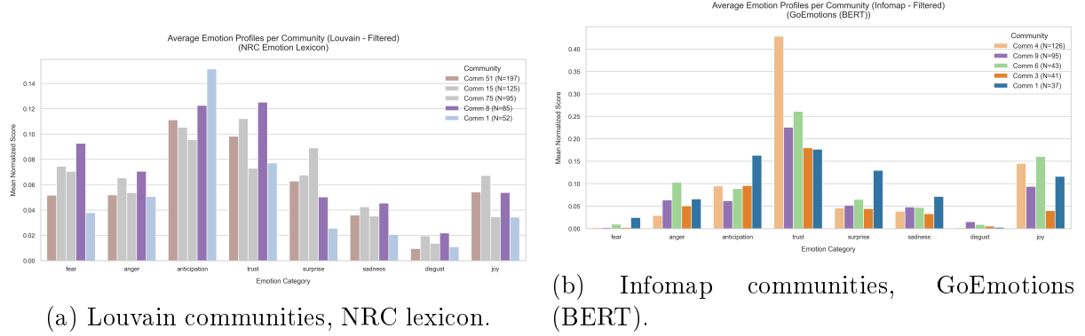
Figure 7: Average emotion profiles for the top communities. Anticipation and trust dominate across clusters; negative emotions stay low.
