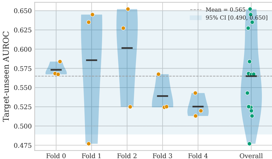
5-Fold Cross-Validation (3 seeds/fold)
