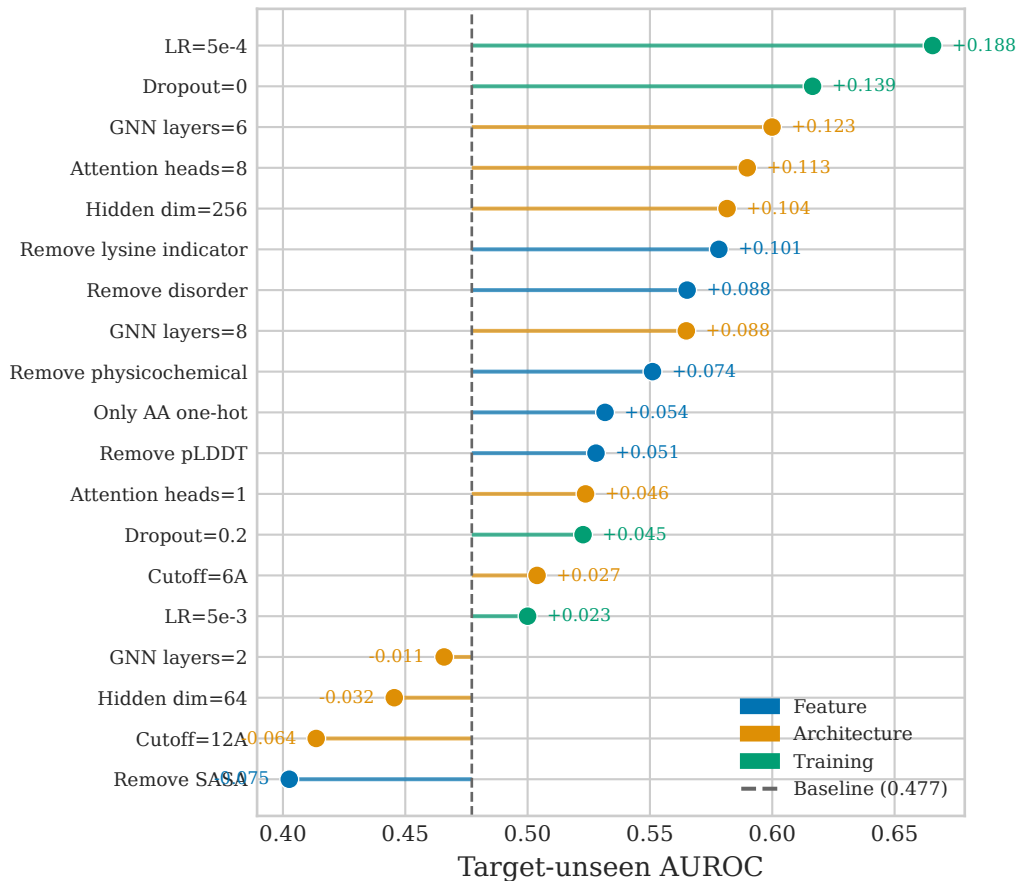
Ablation Study: Effect on Test AUROC
