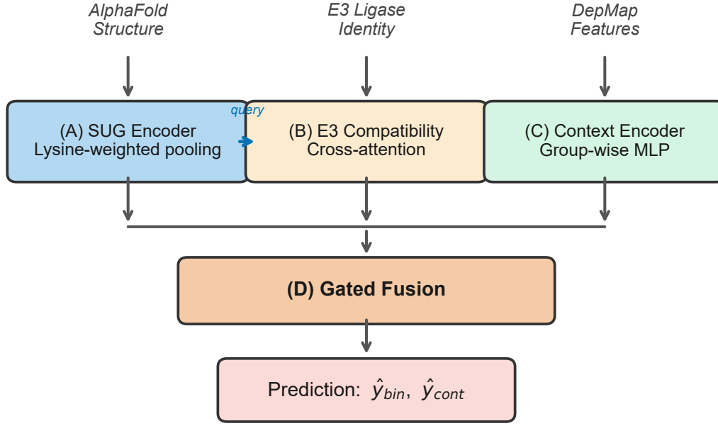
Figure 1: Architecture of SUGNET. Module A (SUG) encodes the protein structure graph with lysine-weighted pooling. Its output serves as the query for Module B’s cross-attention with E3 ligase embeddings. Module C encodes cellular context from DepMap features. Module D fuses all representations through learned gating and produces binary degradability ( \hat{y}_{bin} ) and continuous efficiency ( \hat{y}_{cont} ) predictions.
