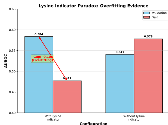
Figure 6: Lysine indicator paradox: removing the lysine indicator improves test performance (+0.101) despite hurting validation (-0.043), revealing a classic overfitting pattern (validation gap: -0.106 vs +0.038).
