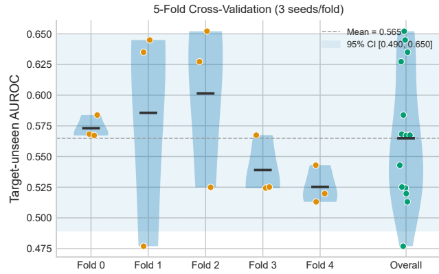
Figure 7: 5-fold cross-validation AUROC distribution. Each dot represents one seed; horizontal bars show fold means. The shaded band indicates the 95% CI of the overall mean (0.565). High inter-fold variance reflects the influence of protein composition on measured performance.
