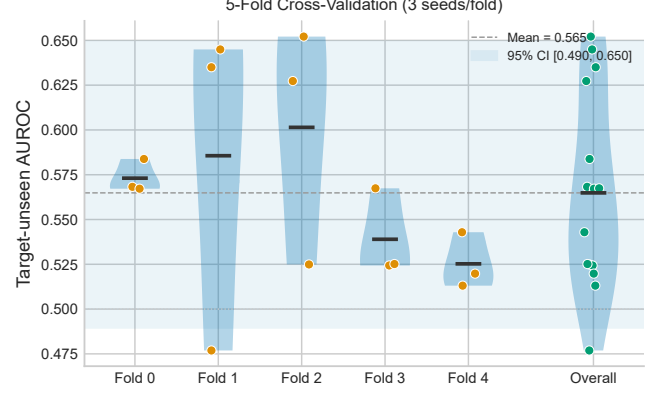
Figure 6: 5-fold cross-validation AUROC distribution. Each dot represents one seed; horizontal bars show fold means. The shaded band indicates the 95% CI of the overall mean (0.565). High inter-fold variance reflects the influence of protein composition on measured performance.
