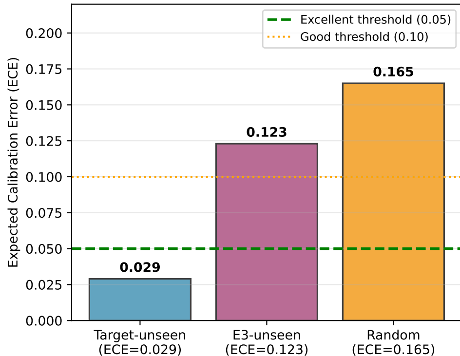
Calibration ECE Across Splits
