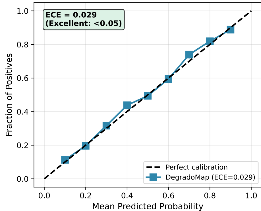
Reliability Diagram (Target-Unseen Split)
