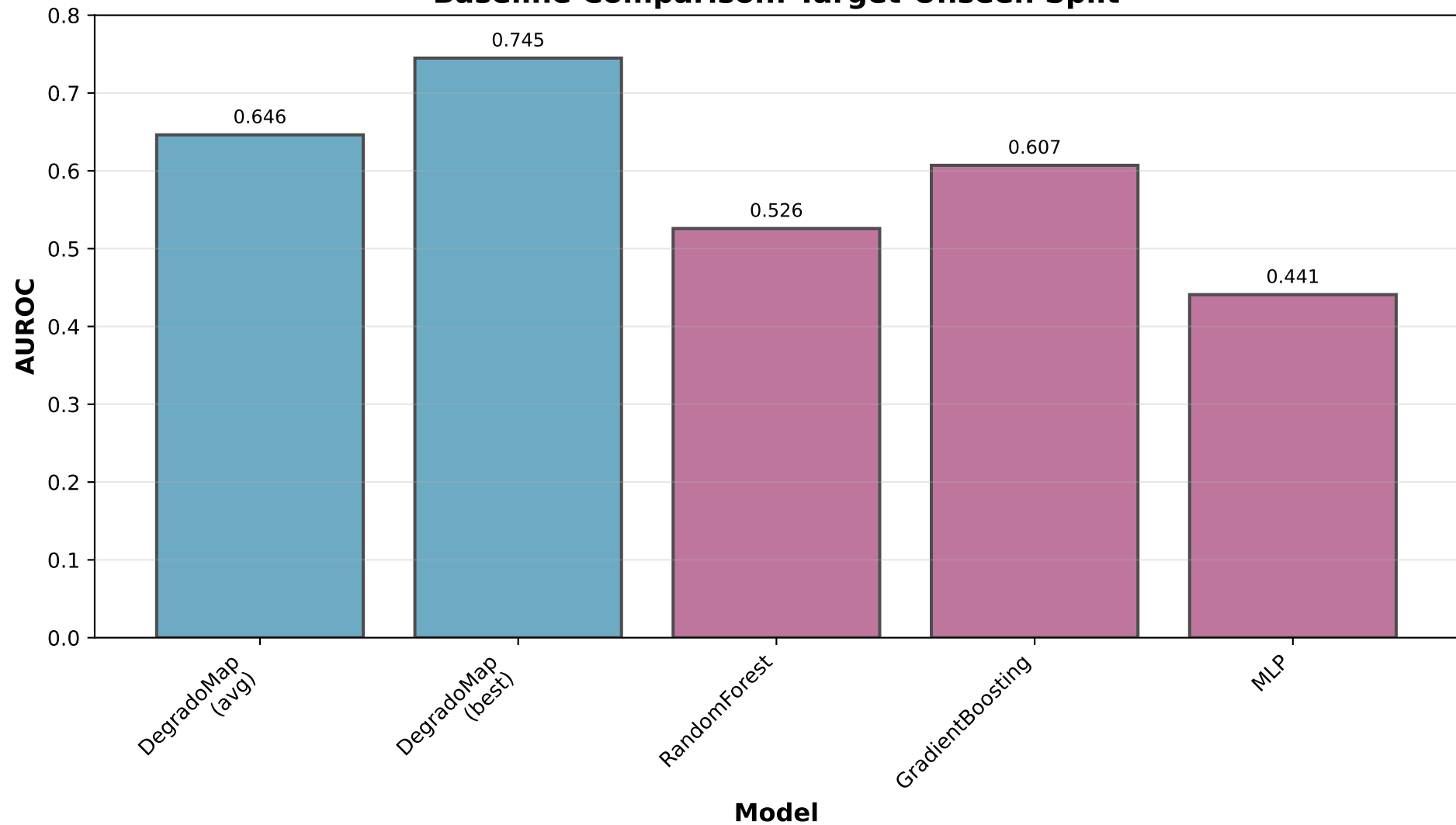
Baseline Comparison: Target-Unseen Split
