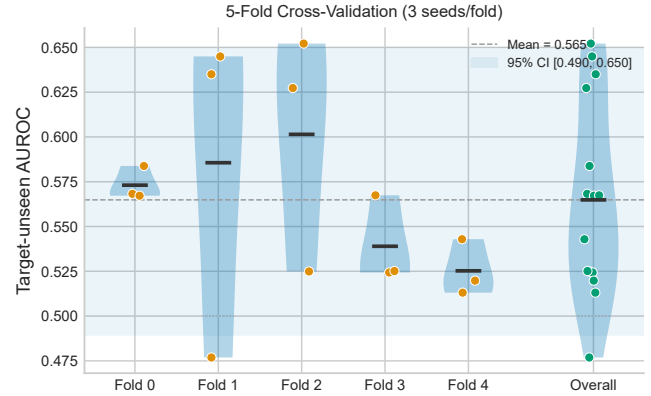
Figure 4: 5-fold cross-validation AUROC distribution. Each dot represents one seed; horizontal bars show fold means. The shaded band indicates the 95% CI of the overall mean (0.565). High inter-fold variance reflects the influence of protein composition on measured performance.
