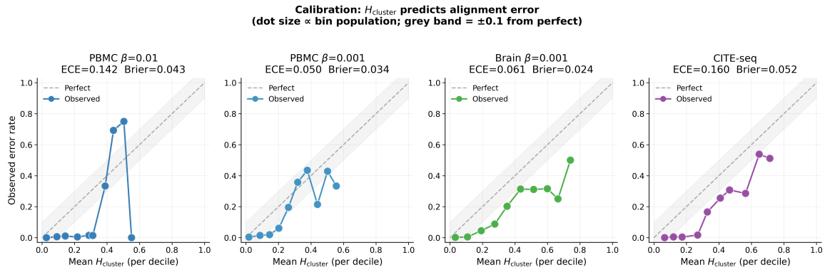
Figure 9: Supplementary Fig. S4: Calibration curves. Mean H_{\text{cluster}} per decile vs. observed error rate: monotonically increasing on all datasets (expected calibration error 0.05–0.16). Multi-seed Brier scores 0.024–0.052.
