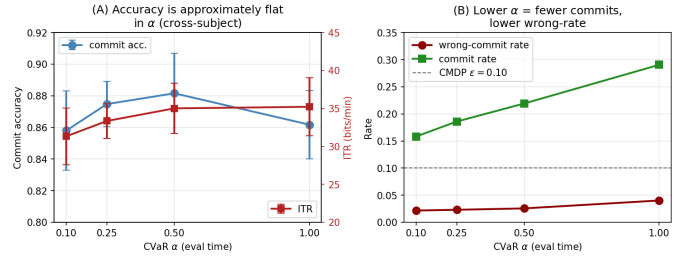
Fig. 6. CVaR \alpha sensitivity on the canonical 3-subject BCI-IV-2a panel (3 subj \times 5 seeds, eval-time sweep over a single distributional-CQL+CMDP \epsilon = 0.10 training). (A) Commit accuracy (blue) and ITR (red) are approximately flat in \alpha . (B) Wrong-commit rate (dark red, 0.022 \rightarrow 0.040 ) and commit rate (green, 0.16 \rightarrow 0.29 ) both double from \alpha = 0.10 to \alpha = 1.00 . The CMDP constraint ( \epsilon = 0.10 , dashed) is comfortably satisfied at every \alpha . \alpha is therefore an operating-point knob, not a no-op.
