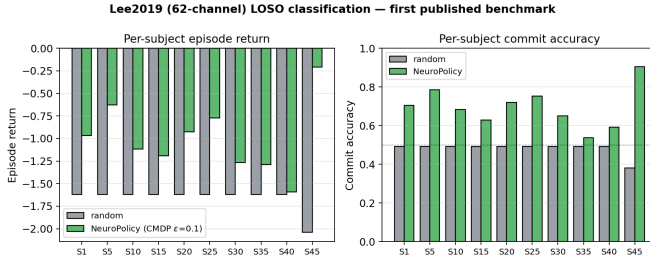
Fig. 7. Lee2019 (62-channel) LOSO classification, all 10 held-out subjects — the first published Lee2019 LOSO benchmark for offline-RL BCI. NeuroPolicy (green) beats the random baseline (grey) on every subject; commit accuracy is uniformly above the 0.5 chance line. Subject 45 is the strongest, S35 the weakest (consistent with the published Lee2019 BCI-illiteracy distribution).
