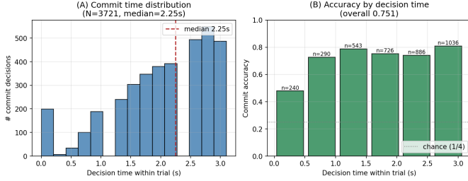
Fig. 5. When the selective decoder commits within a trial, pooled across 9 BCI-IV-2a subjects \times 5 seeds \times 2 configs ( N = 3721 commit decisions); median decision time 2.25 s ( \sim 56\% of full trial length). (A) Commit-time distribution is bimodal: \sim 6\% of decisions fire immediately at the first step (impulsive-commit mode), the bulk ( \sim 85\% ) cluster between 1.25–3.0 s as the value head accumulates evidence, and very few fire in the 0.5–1.0 s window. (B) Commit accuracy by decision-time bin: early-impulse commits ( \leq 0.5 s) drop to 0.48, while every later bin ( \geq 1 s) is above 0.73, the expected speed-accuracy trade-off. Overall pooled commit accuracy 0.751.
