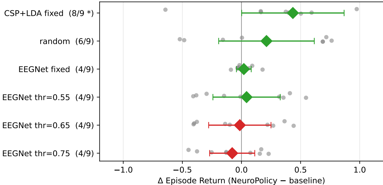
LOSO BCI-IV-2b — paired difference vs. baselines (diamond = mean, error bar = 95% CI; * = Wilcoxon p < 0.05 )
