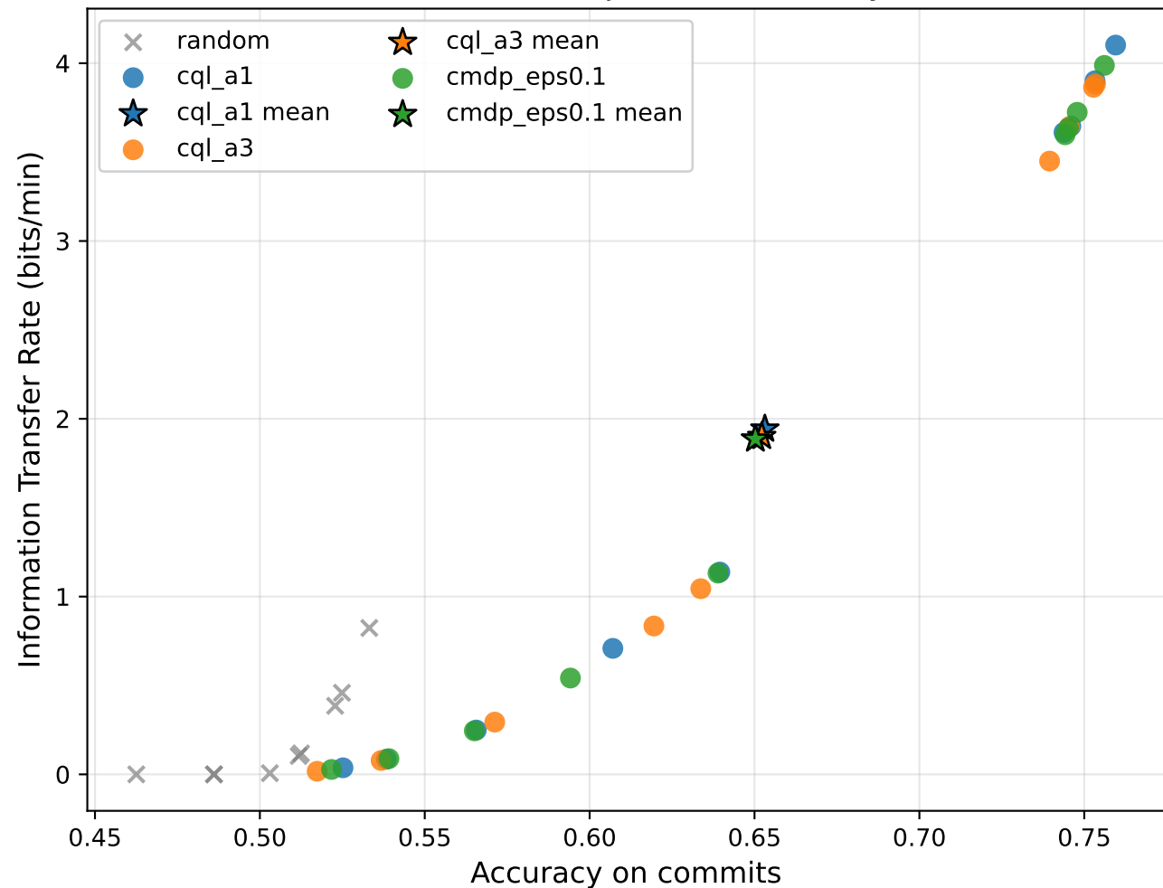
BCI-IV-2b LOSO (9 subjects) — accuracy vs ITR
