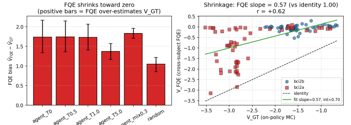
Fig. 7. Fitted-Q estimator shrinks toward zero on the N=9 LOSO OPE corpus. Linear fit V_{FQE} = 0.57 V_{GT} + 0.70 ( r = +0.62 ); weak-decodability subjects (red) exhibit 44% larger shrinkage.
