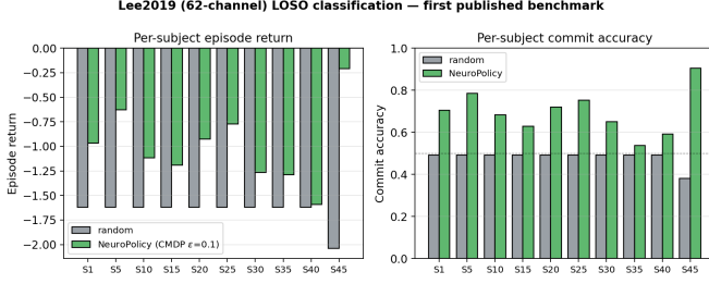
Fig. 5. Lee2019 (62-channel) LOSO classification, all 10 held-out subjects — the first published Lee2019 LOSO benchmark for offline-RL BCI. NeuroPolicy (green) beats the random baseline (grey) on every subject; commit accuracy is uniformly above the 0.5 chance line. Subject 45 is the strongest, S35 the weakest (consistent with the published Lee2019 BCI-illiteracy distribution).
