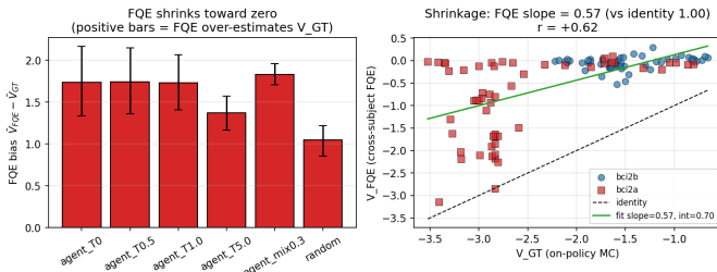
Fig. 7. Fitted-Q estimator shrinks toward zero on the N=9 LOSO OPE corpus. Linear fit V_{\text{FQE}} = 0.57 V_{\text{GT}} + 0.70 ( r = +0.62 ); weak-decodability subjects (red) exhibit 44% larger shrinkage.
