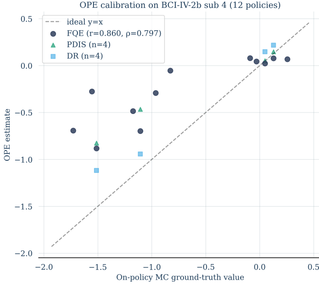
Fig. 1. Off-policy evaluation calibration on BCI-IV-2b subject 4. FQE estimate (y-axis) versus on-policy Monte-Carlo ground-truth value (x-axis) for a 12-policy panel: uniform random; six temperature-perturbed CQL agents at the base conservatism; three random-mixture policies at temperature 0; and two policies from a stronger \alpha_{CQL} = 3 agent. FQE achieves Pearson r = 0.860 ( p = 3.3 \times 10^{-4} ), Spearman \rho = 0.797 , RMSE = 0.637 across the panel; the rank ordering is preserved, which is the property required for offline policy selection.
